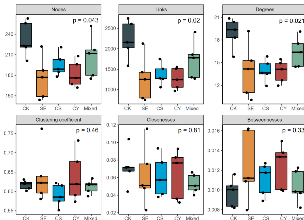
Figure 4. Comparison of node-level topological feature of gut bacterial community co-occurrence patterns among control and the TCM feeding groups. CK: control, SE: Semen euryales, CS: Coix seed, CY: Chinese yam, Mixed: both of Semen euryales, Coix seed and Chinese yam
