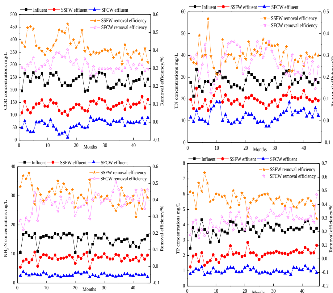
Figure 3. The removal performance of COD, TN, TP and NH 3 -N
