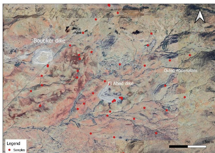
Figure 2. Surface of sampling sites of soils, sediments and mining wastes collected from El Abed area
