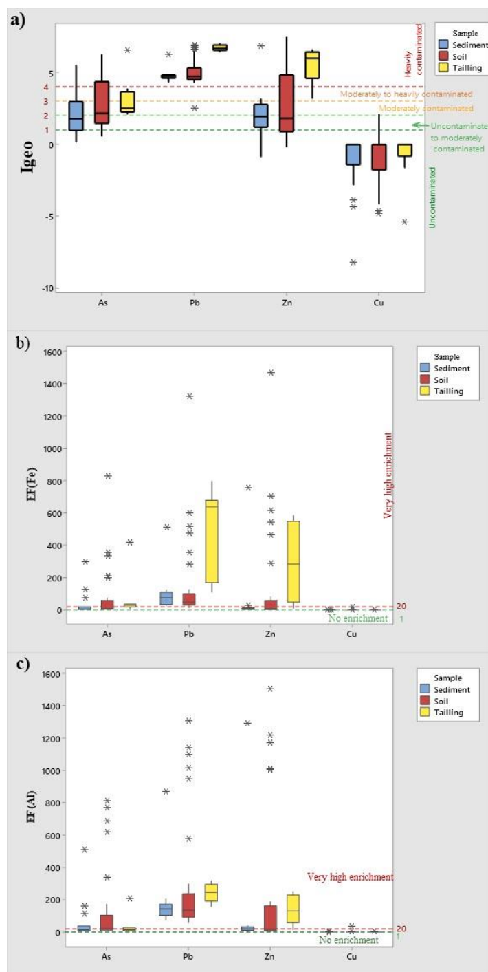
Figure 5. Box plot for mean geoaccumulation index ( I_{geo} ), mean enrichment factors (EF) with iron and aluminum references for trace elements (Pb, As, Zn and Cu) in the studied soil, sediment and mining waste samples of the region El Abed (classification reference values shown by horizontal dashed lines)
