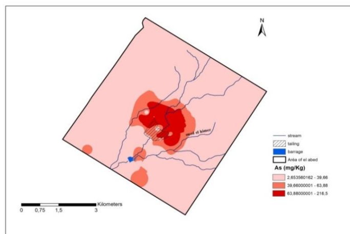
Figure 8. Spatial distribution map of the trace metal arsenic in the soils, sediments and mining wastes of El Abed area
