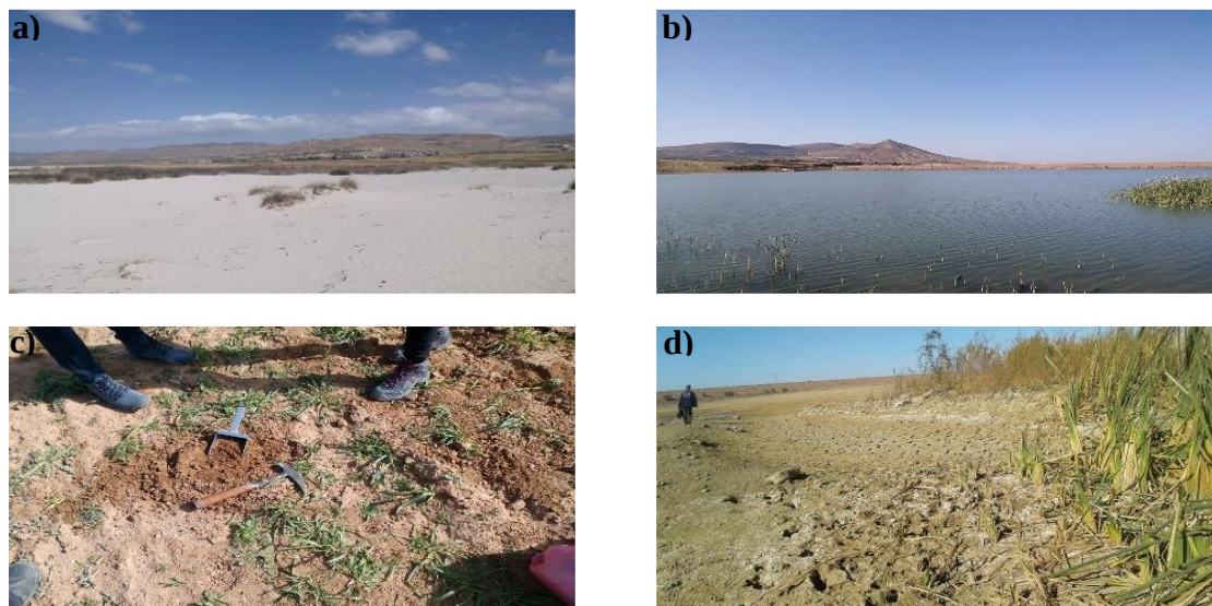
Figure A1. Photos showing the the tailings dyke stored in the open area (a), the general view of the dam and the mine (b) and sampling areas (c and d)
