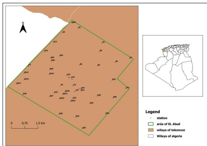
Figure 1. The location of the El Abed region in relation to the map of Algeria and sampling sites
