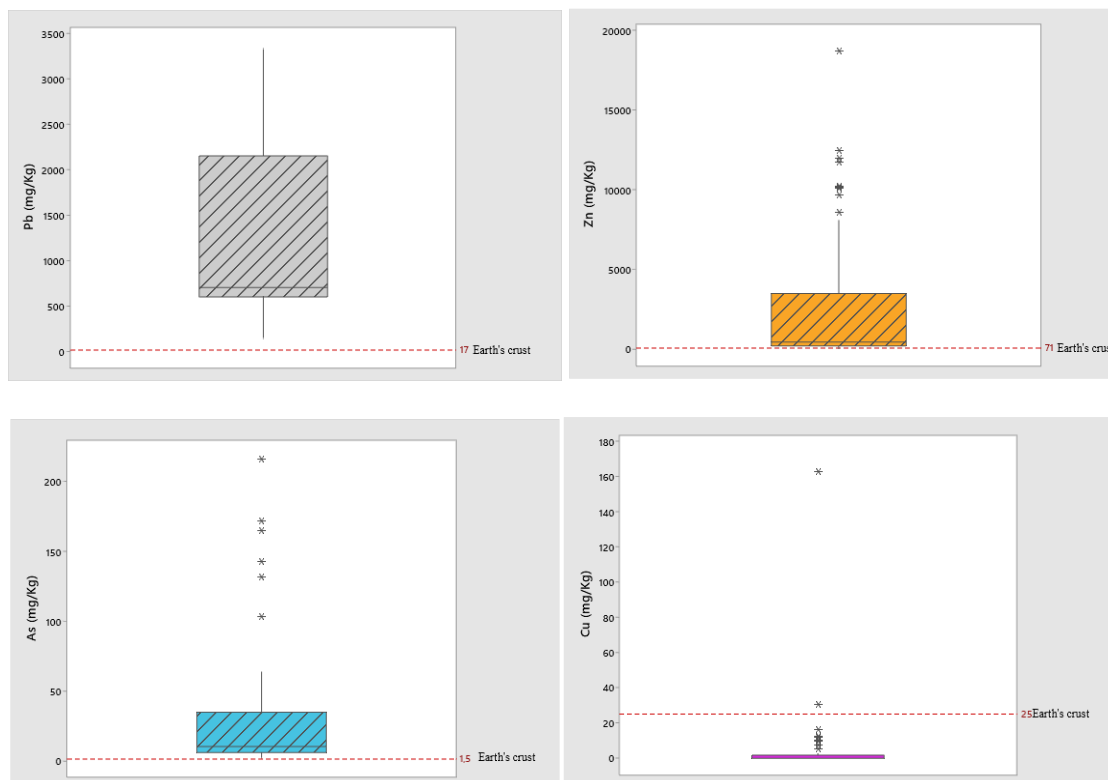
Figure 3. Box plot for trace metals (Pb, Zn, As and Cu) concentrations in the El Abed
