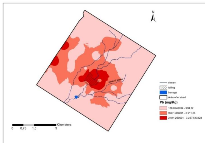
Figure 7. Spatial distribution map of the trace metal lead in the soils, sediments and mining wastes of El Abed area
