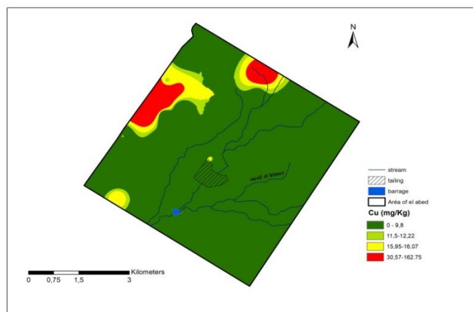
Figure 9. Spatial distribution map of the trace metal copper the soils, sediments and mining wastes of El Abed area
