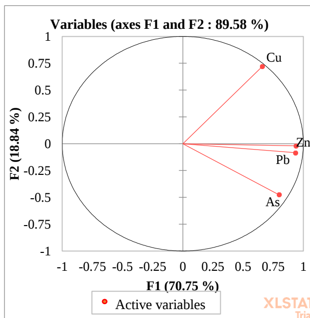
Figure 4. Representation of the results of the analysis of the main component of the surface samples of El Abed area projecting the variables (trace metals) on the level F1-F2
