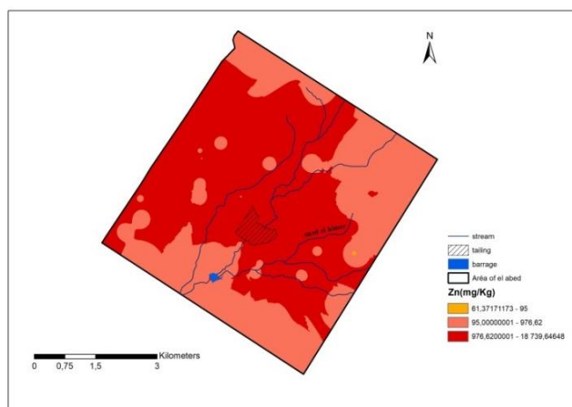
Figure 6. Spatial distribution map of the trace metal zinc in the soils, sediments and mining wastes of El Abed area
