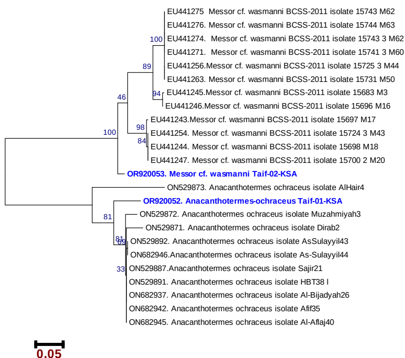
Figure 2. The maximum likelihood method phylogenetic tree is based on the Tamura-Nei model (Tamura and Nei, 1993). The tree was constructed based on the partial sequence of COI of both termites (591 nts) and black ants (480 nts) collected from the Taif region. International and local sequences from the Genbank database were used to confirm the identity of our collected insects and their genetic relatedness with other sequences of the same species. Insect species used in the current study are shown in blue fonts and bootstrapping values are shown above the branches
