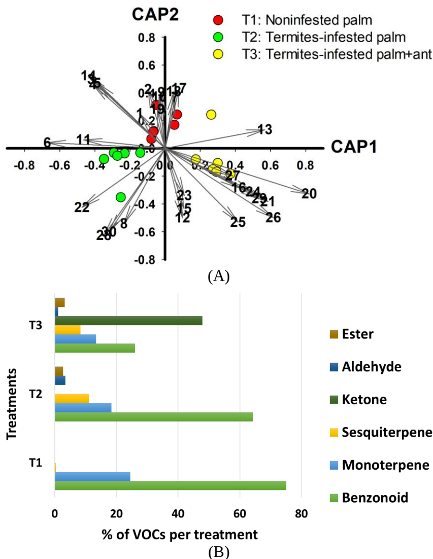
Figure 3. (A) CAP analysis of the headspace compounds ( n = 30 ) released by non-infested date palm trees T1(red), termite-infested date palm trees T2(green) and termite-infested palm after adding ant T3(yellow) analyzed by GC/MS ( n = 18 samples), two canonical axes of the canonical analysis of principle coordinates (CAP) analysis are plotted. CAP analysis demonstrates the separation of the samples based on the presence and absence of headspace compounds. Scaled vectors of the headspace compounds (ID numbers) were significant ( |r| > 0.2 ) for the separation of the groups, miss-classification error = 9.52%. The numbers refer to the headspace compounds in Table 1 . (B) A histogram displays the emissions percentage of VOCs released in the chemosphere of three date palm treatments (T1, T2 and T3)
