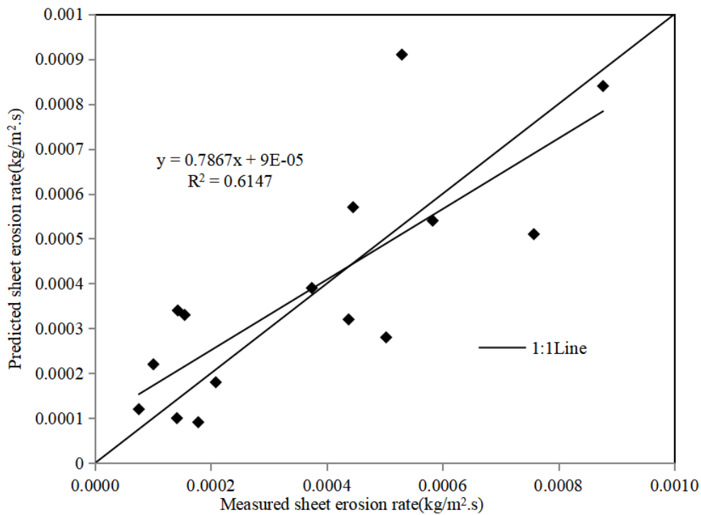
Figure 1. Measured versus modeled SE ( SE = 1.26 \times 10^{-8} I^{2.52} q^{-0.74} )
