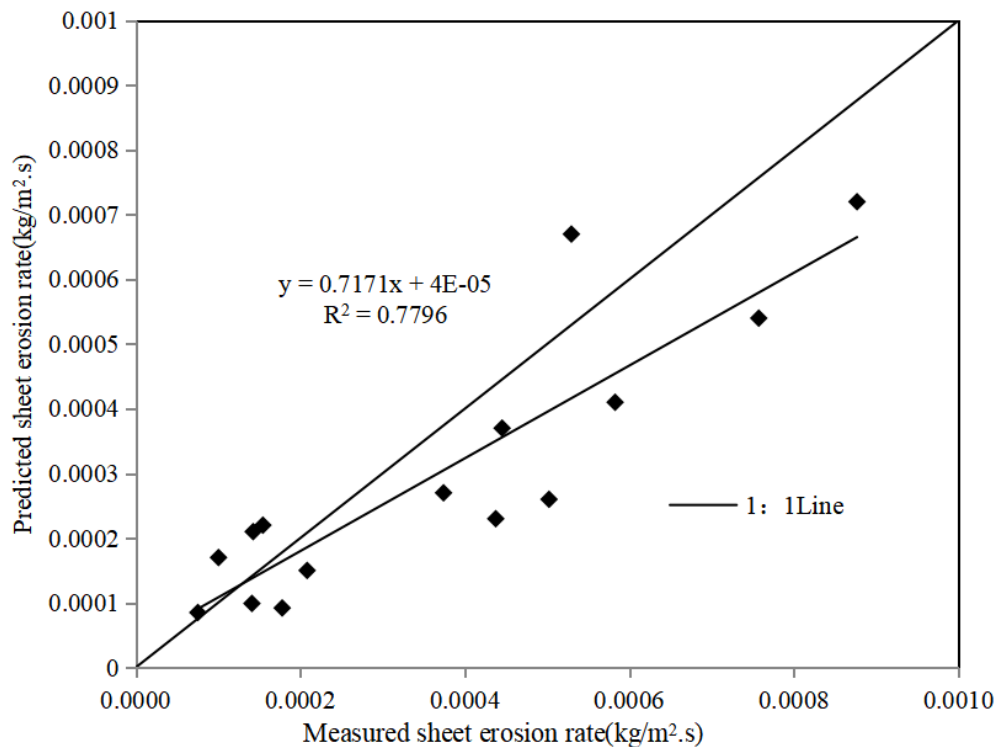
Figure 2. Measured versus modeled SE ( SE = 1.66 \times 10^{-13} I^{3.54} q^{-1.55} C^{-0.89} )
