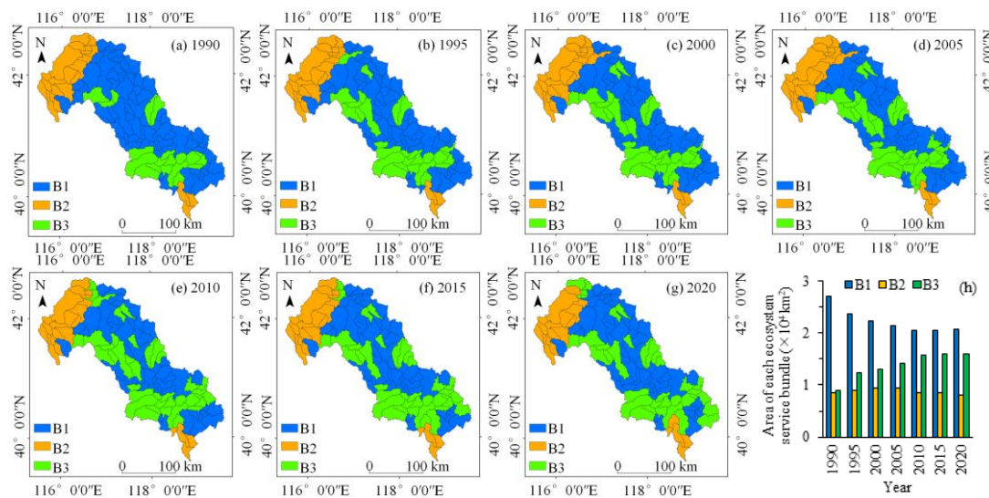
Figure 7. (a–g) Spatial distribution of ecosystem services bundles in the Luan River Basin from 1990 to 2020. (h) Temporal distribution of ecosystem services bundles in the Luan River Basin from 1990 to 2020
