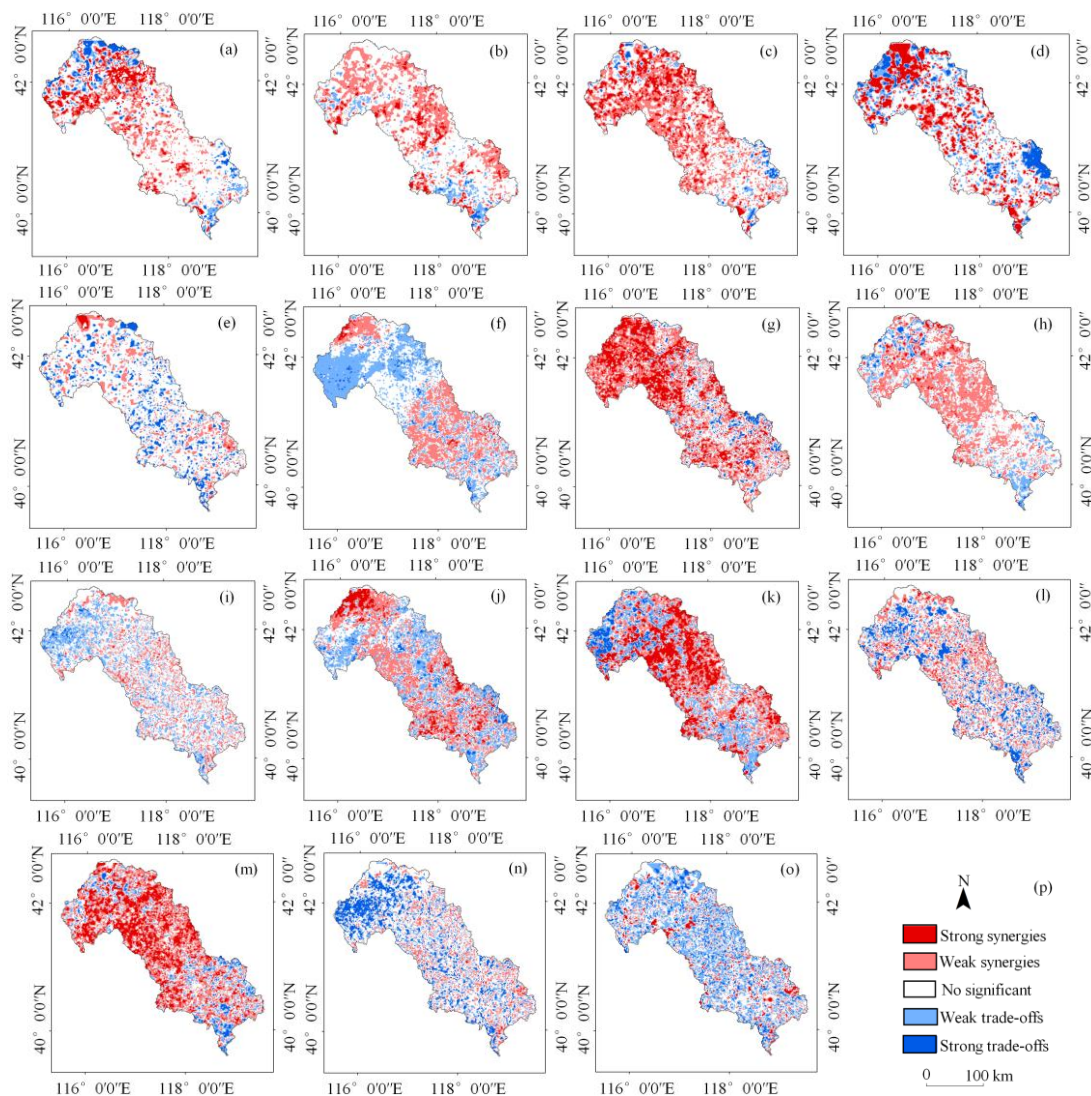
Figure 5. Spatial distribution of trade-offs and synergies between ecosystem services: (a) carbon storage and water yield; (b) carbon storage and soil conservation; (c) carbon storage and water retention; (d) carbon storage and habitat quality; (e) carbon storage and food supply; (f) water yield and soil conservation; (g) water yield and water retention; (h) water yield and habitat quality; (i) water yield and food supply; (j) soil conservation and water retention; (k) soil conservation and habitat quality; (l) soil conservation and food supply; (m) water retention and habitat quality; (n) water retention and food supply; and (o) habitat quality and food supply
