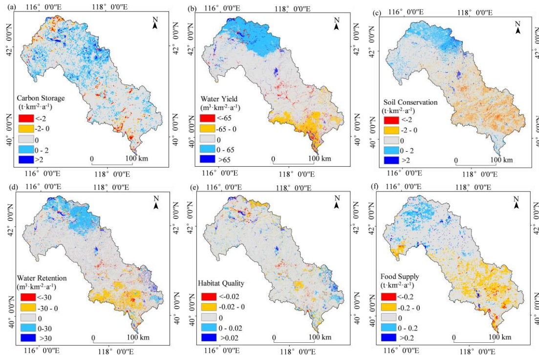
Figure 2. Spatial variability of the values for individual ecosystem services in the Luan River Basin from 1990 to 2020: (a) carbon storage; (b) water yield; (c) soil conservation; (d) water retention; (e) habitat quality; and (f) food supply
