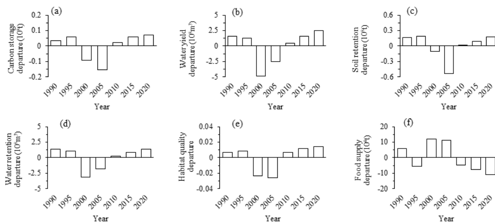
Figure 3. Departure of the values obtained for individual ecosystem services in the Luan River Basin from 1990 to 2020: (a) carbon storage; (b) water yield; (c) soil conservation; (d) water retention; (e) habitat quality; and (f) food supply
