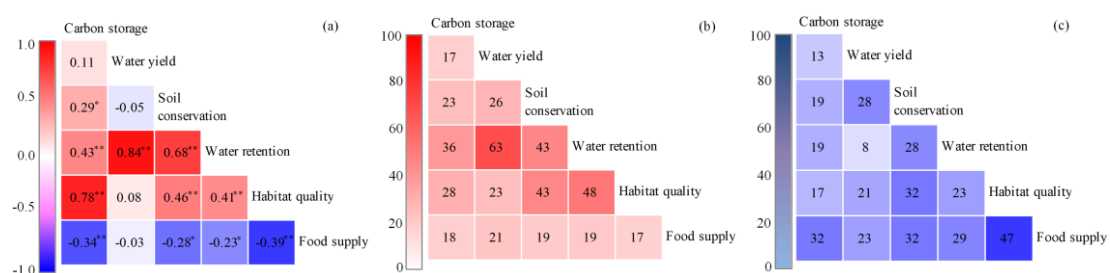
Figure 4. (a) Matrix of Pearson correlations between different ecosystem services (* p < 0.05 ; ** p < 0.01 ). Red and blue colors indicate positive and negative correlations, respectively. The deeper the color, the higher the correlation. (b) Proportion of area for synergies between ecosystem services (%). (c) Proportion of area for trade-offs between ecosystem services (%)
