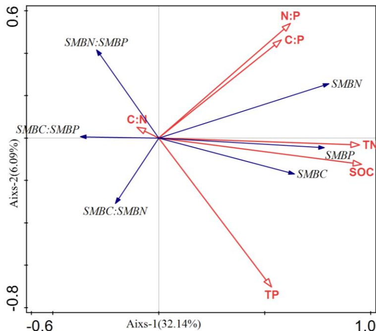
Figure 4. Redundancy analysis (RDA) was used to identify the associations between microbial biomass stoichiometry and soil properties
