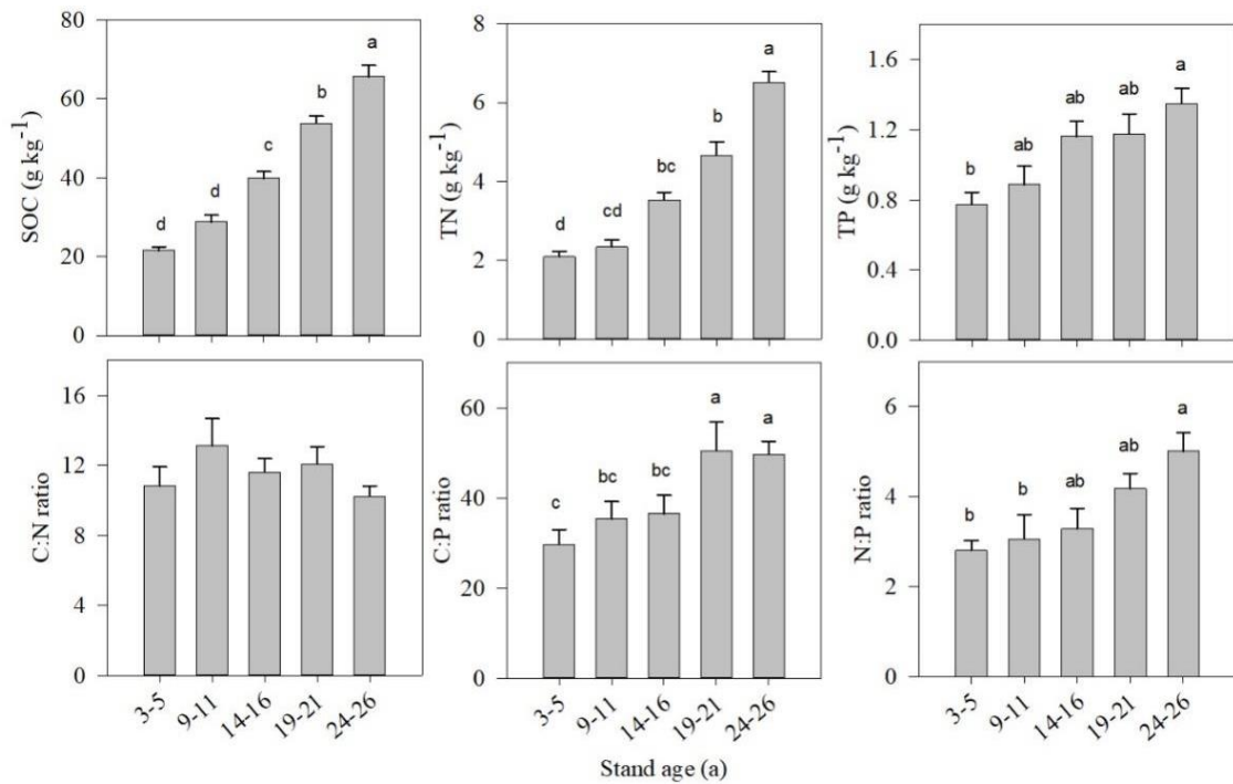
Figure 2. Changes in SOC, TN, TP, and stoichiometric ratios of soil C:N, C:P and N:P during vegetation succession in a karst region of Southwest China. The values are the means \pm SE ( n = 8 ). The different lowercase letters on the columns denote significant differences between successional stages at p < 0.05
