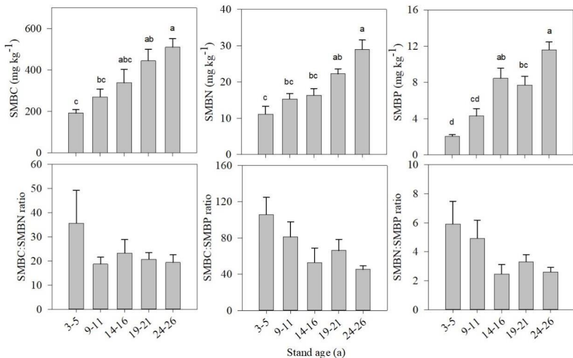
Figure 3. Changes in SMBC, SMBN, SMBP, and stoichiometric ratios of SMBC:SMBN, SMBC:SMBP and SMBN:SMBP during vegetation succession in a karst region of Southwest China. The values are the means \pm SE ( n = 8 ). The different lowercase letters on the columns denote significant differences between successional stages at p < 0.05
