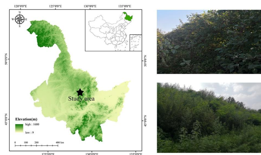
Figure 1. Sample plot and diagram of the experimental design in Wuying national nature reserve, Yichun city, Heilongjiang province, northeastern China
