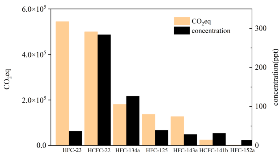
Figure 2. CO 2 -equivalent GWP and concentrations of species at Gosan Station in 2020
