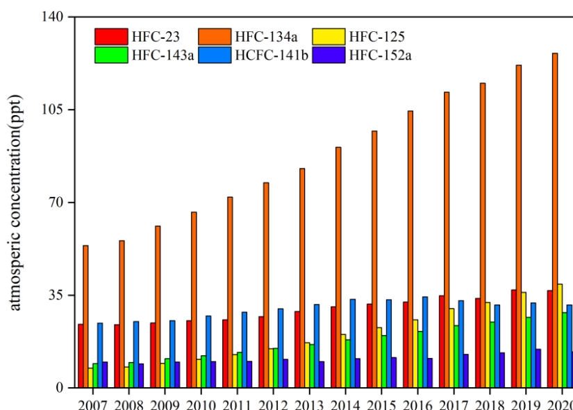
Figure 3. FGHG Concentration Trends at Gosan Station from 2007 to 2020
