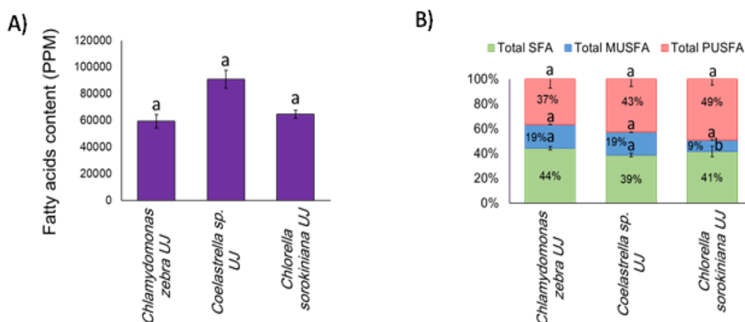
Figure 3. Fatty acid content of microalgae isolates. (A) Total fatty acids content calculated as ppm. (B) Distribution of each class of fatty acids
