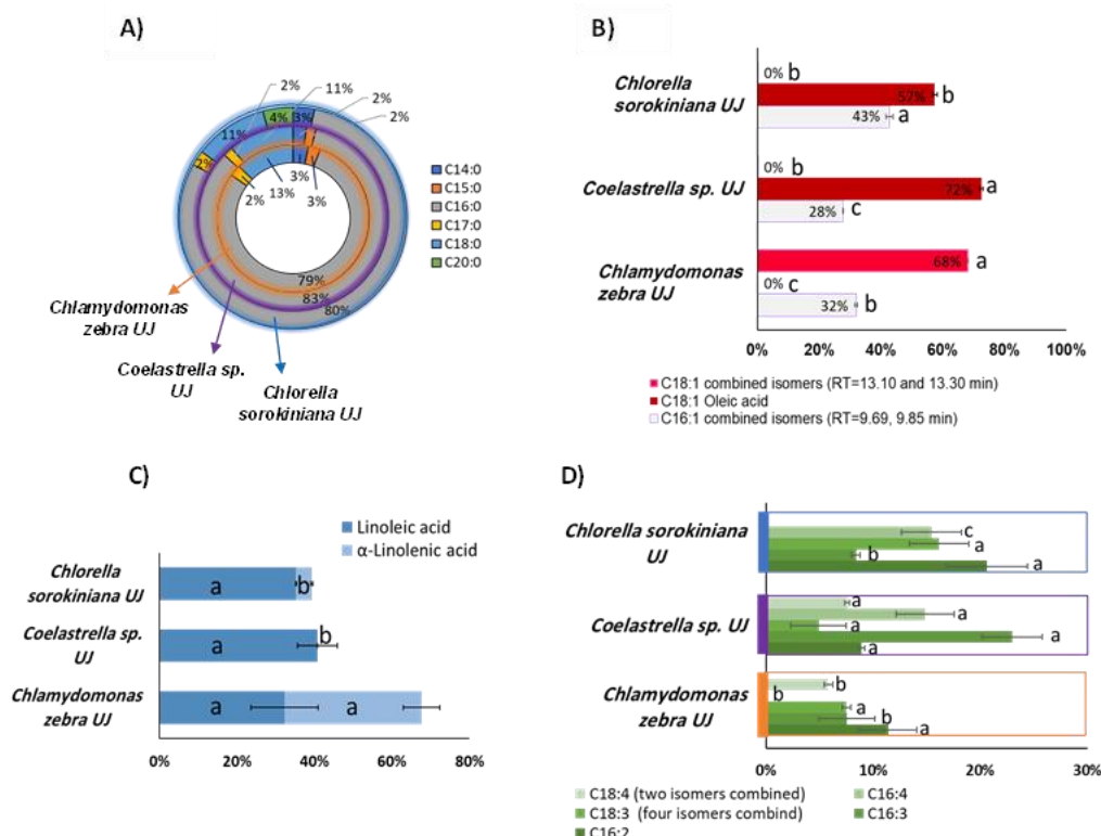
Figure 4. Distribution of different classes of fatty acids. (A) Percentage of different saturated fatty acids relative to the total saturated fatty acids. (B) Percentage of monounsaturated fatty acids relative to the total monounsaturated fatty acids. (C) Percentage of linoleic acid and α-linolenic acid to the total polyunsaturated fatty acids. (D) Distribution of other unknown polyunsaturated fatty acids to the total polyunsaturated fatty acids
