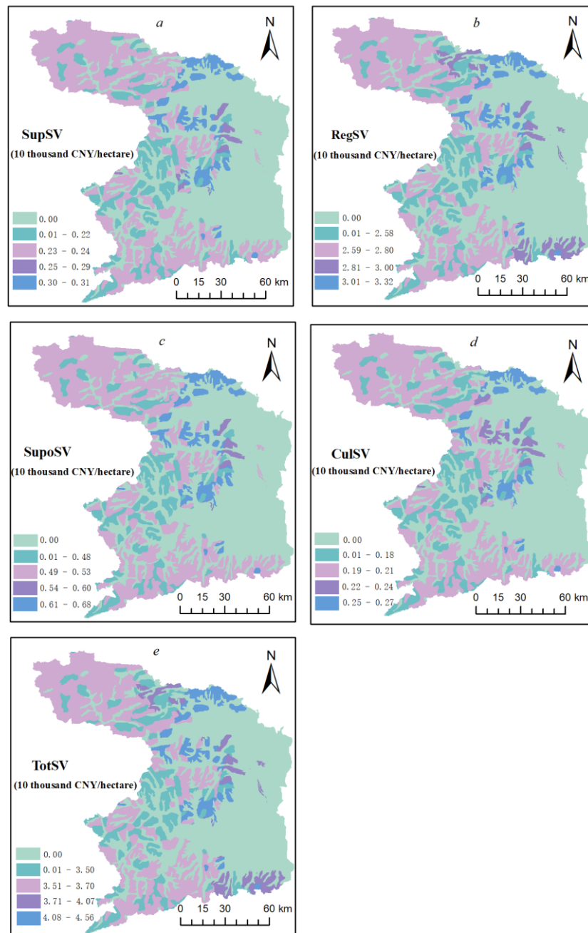
Figure 5. Spatial distribution map of forest ecosystem service value under scale ii in Changde City. SupSV : supply service value, RegSV : regulatory service value, SupoSV : support service value, CulSV : cultural service value, TotSV : the total of service value
