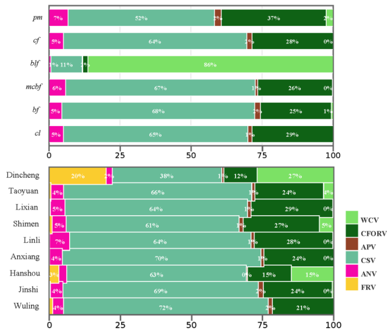
Figure 4. The Value and value composition ratio of forest ecological services in different stands, districts, and counties under Scale I in Changde city. cl : Chinese Fir Forests, pm : Masson Pine Forests, cf : Cypress Forests, blf : Broadleaf Forests, mcbf : Coniferous and Broadleaf Mixed Forests, bf : Bamboo Forests. WCV: water conservation value, CSV: conservation soil value, CFORV: carbon sequestration and oxygen release value, APV: air purification value, ANV: accumulated nutrient value, FRV: forest recreation value
