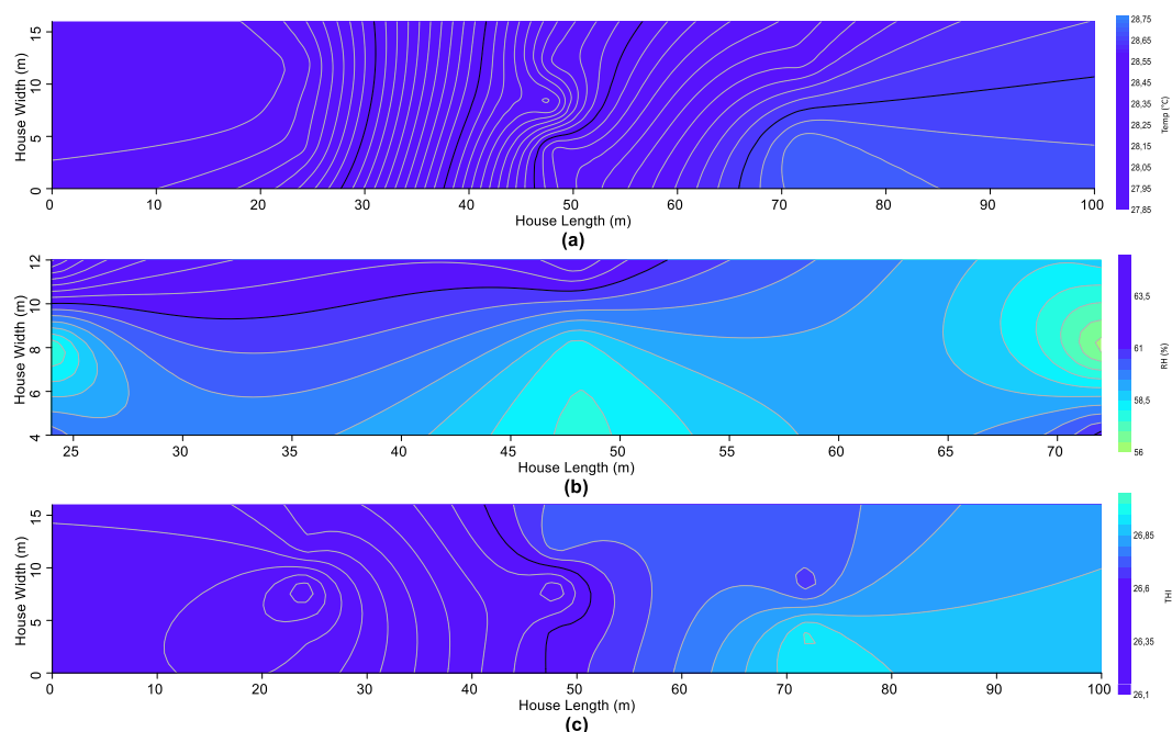
Figure 7. THI distribution estimation map. (a) daily, (b) daytime (c) nighttime
