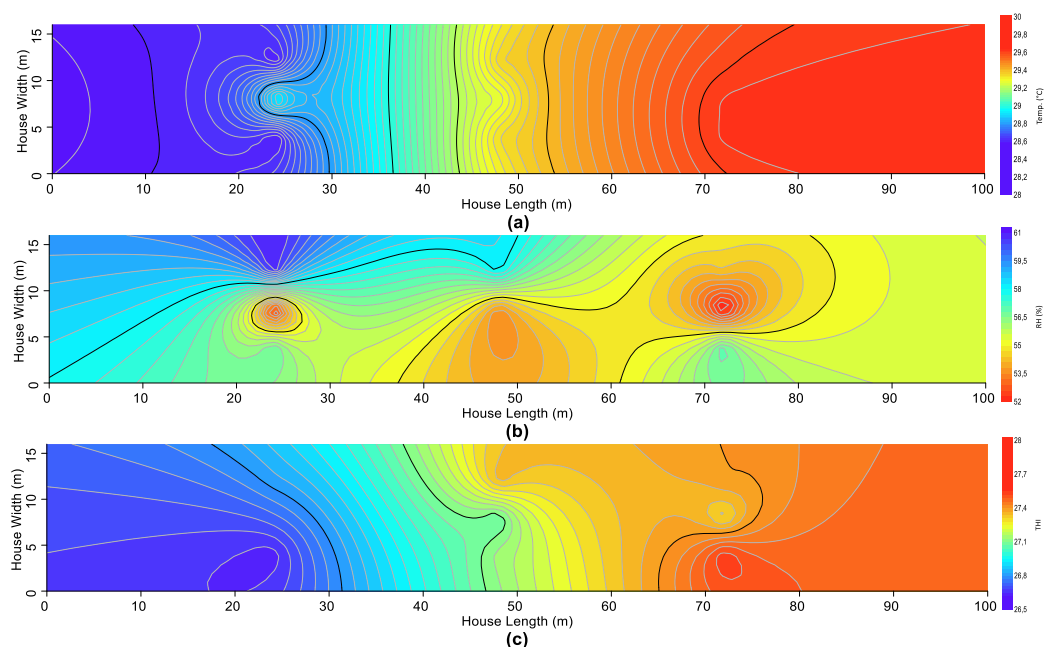
Figure 5. Temperature distribution estimation contour map. (a) daily, (b) daytime (c) nighttime
