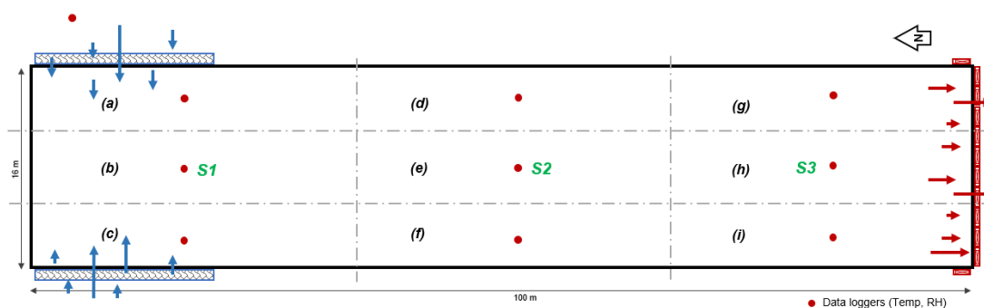
Figure 1. The schematic layout of cooling and ventilation equipment along with data loggers in the broiler house
