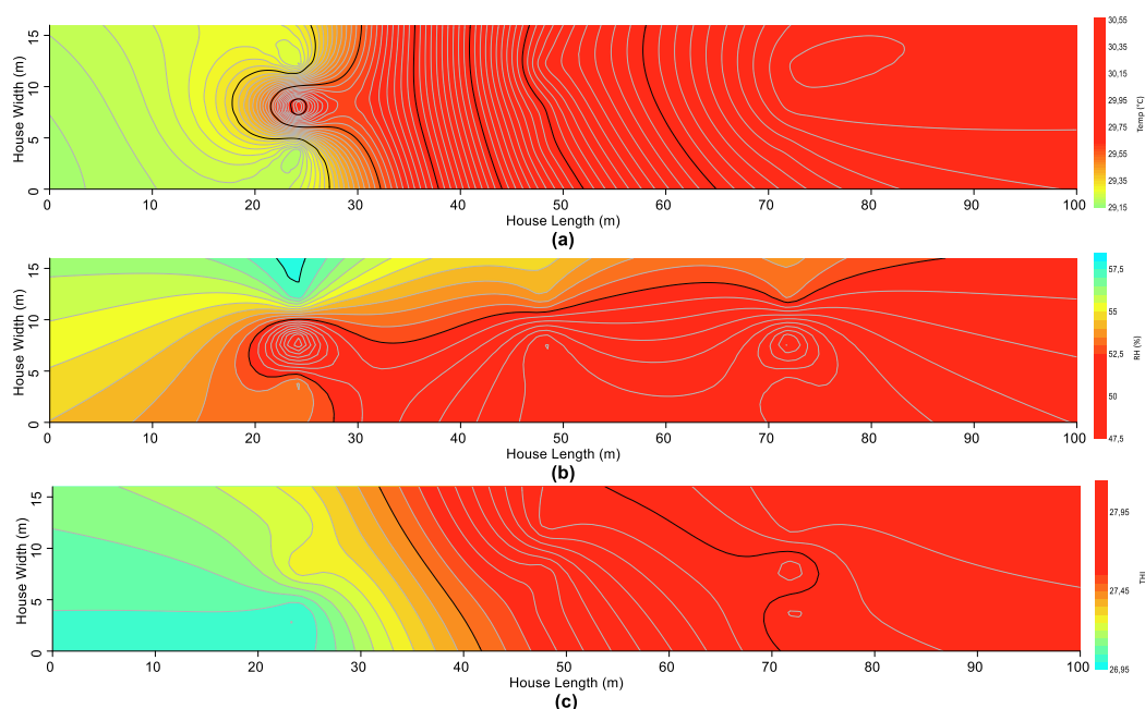
Figure 6. RH distribution estimation contour map. (a) daily, (b) daytime (c) nighttime
