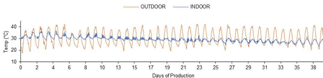
Figure 2. Average daily temperatures in indoor and outdoor environments
