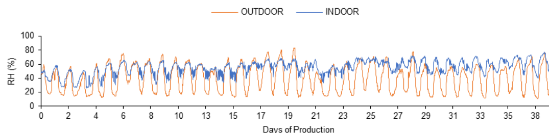
Figure 3. Average daily RH in indoor and outdoor environments
