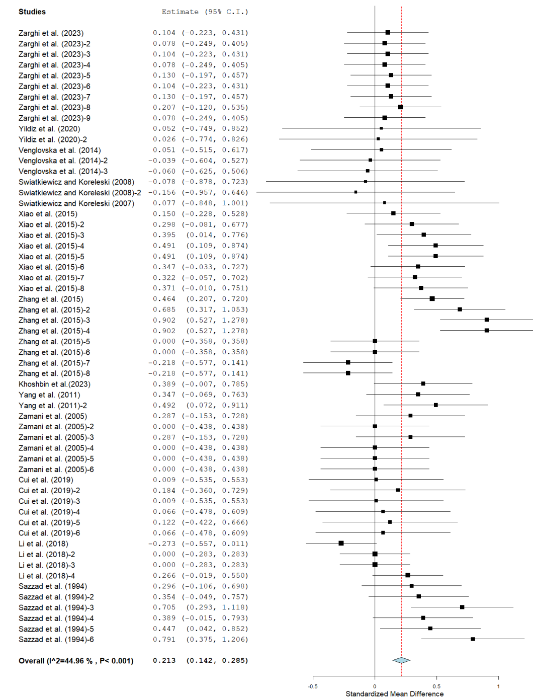
Figure 8. Forest plot of the effect of Mn on EST
