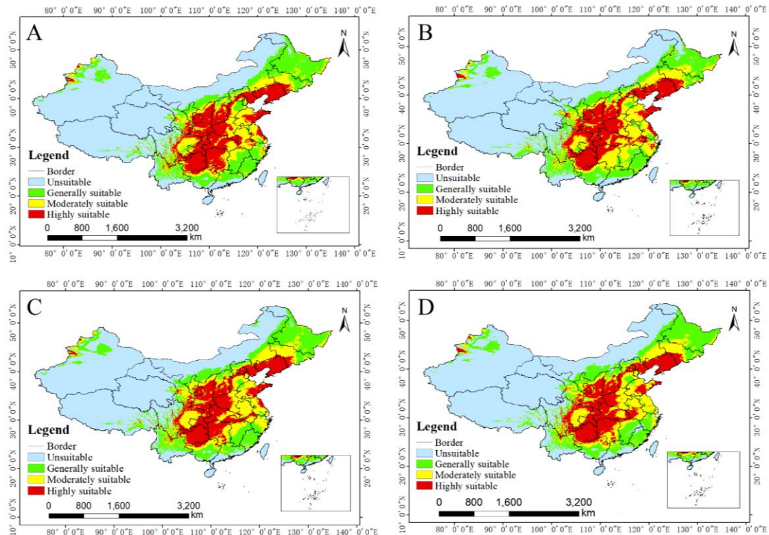
Figure 6. Potential distribution of Lithospermum erythrorhizon under future climate: 2041-2060, SSP 126 (A); 2081-2100, SSP 126 (B); 2041-2060, SSP 585 (C); 2081-2100, SSP 585 (D)
