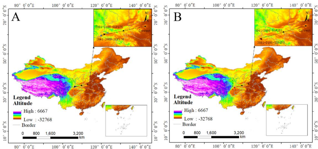
Figure 7. Centroid migration trajectories of the total suitable habitat for Lithospermum erythrorhizon under future climate change: 2050s -2090s, SSP126 (A); 2050s -2090s, SSP585 (B)
