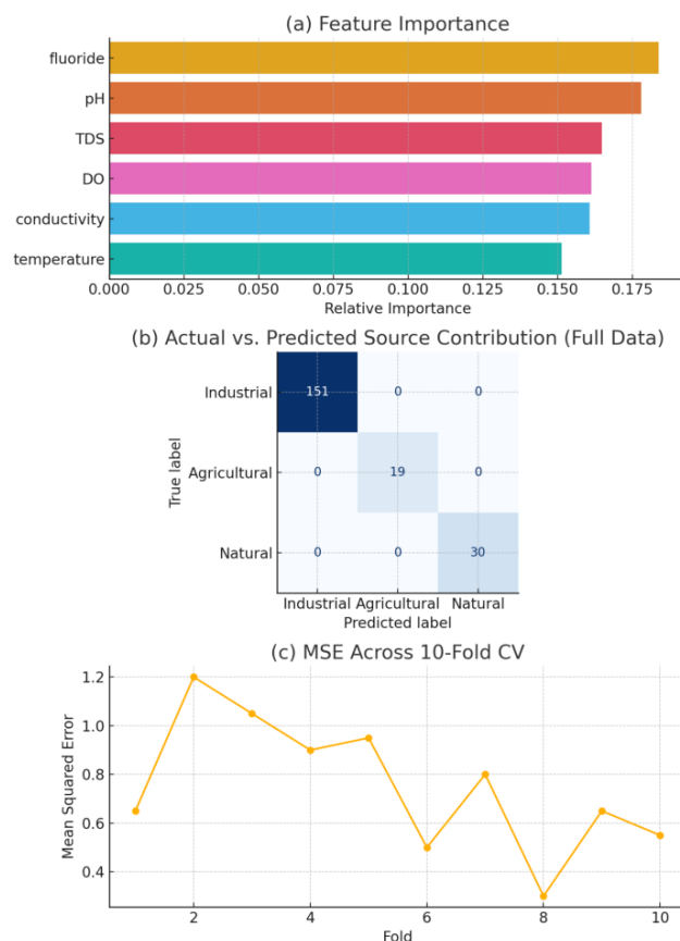
Figure 2. Cross-validation results of the Random Forest model (2010–2024) for fluoride pollution source classification in the Yangtze River Basin. Note: TDS = Total dissolved solids; DO = Dissolved oxygen; MSE = Mean squared error
