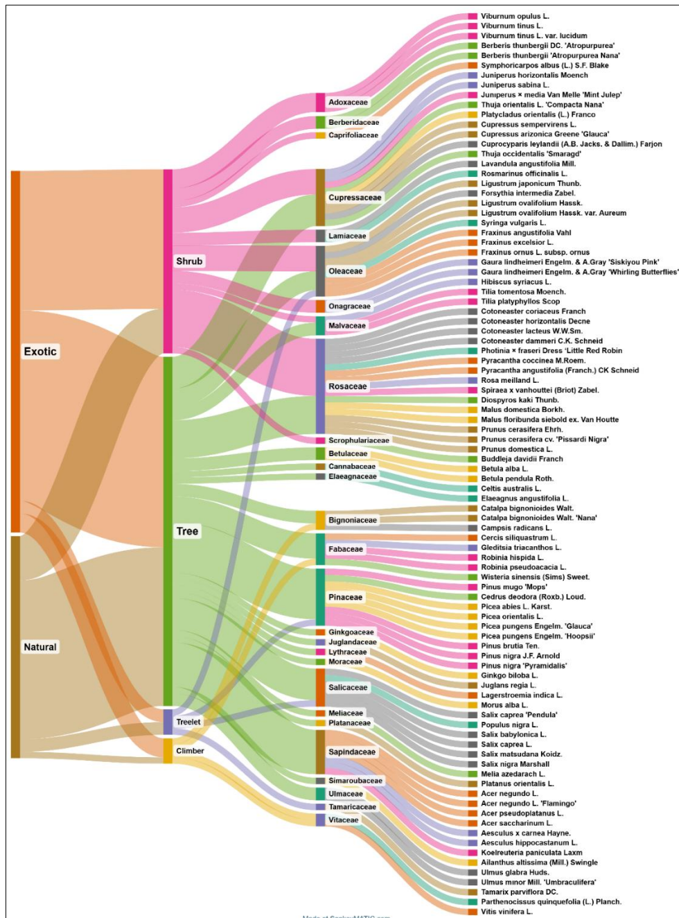
Figure 9. Sankey diagram
