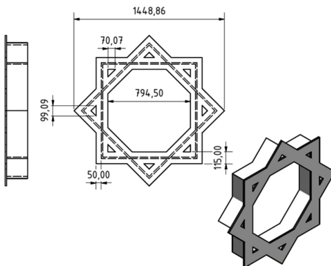
Figure 1. Scheme of the chandelier frame
