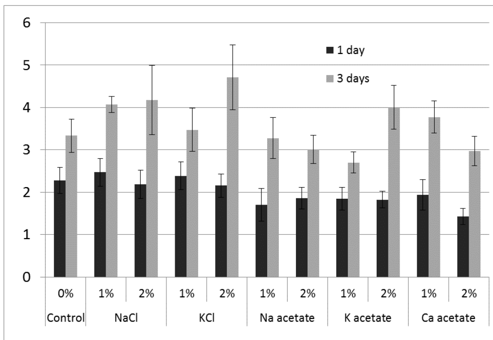
Figure 5. Effects of salt forms and concentrations on the firmness of wheat bread crumb (kg)
