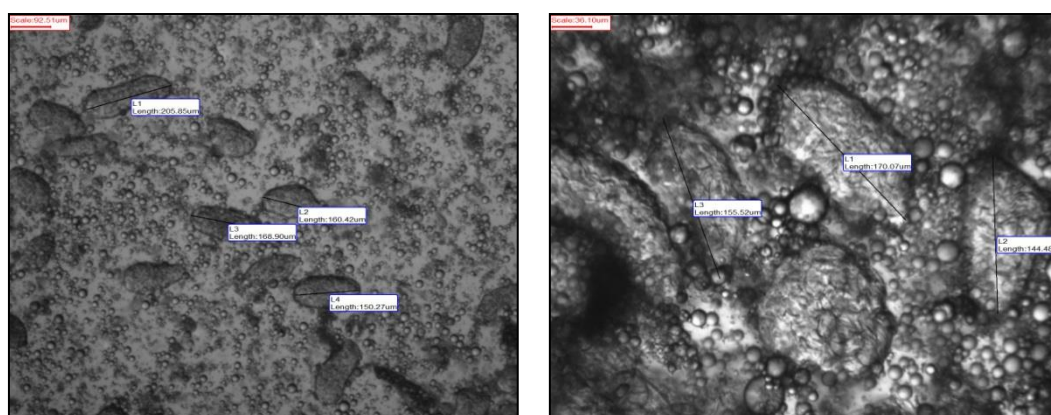
Figure 6. Structure of humus spread with optimal properties and distribution of its constituents
