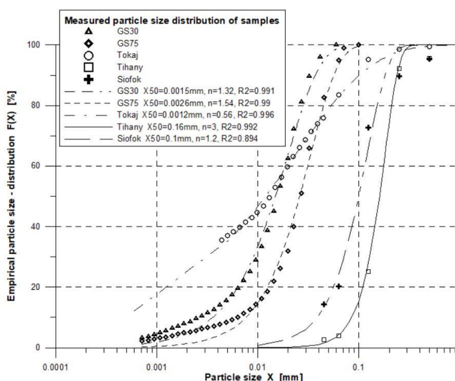
Figure 1. Measured PSD curves of the samples.
