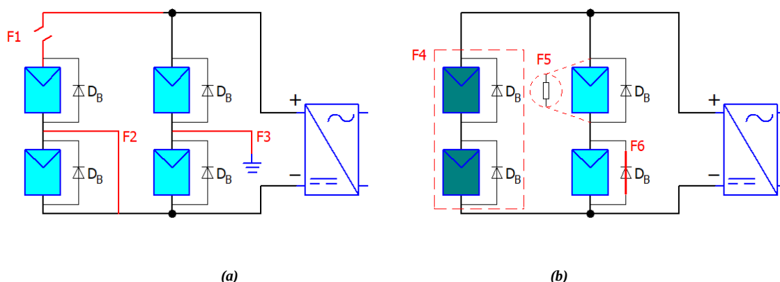
Figure 3. Circuit diagram of the PV system for validation. (a) open-circuit and short-circuit fault and grounding fault (b) partial shading degradation fault and bypass diode fault
