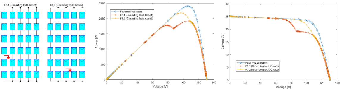
Figure 9. The PV array configuration for Grounding fault
