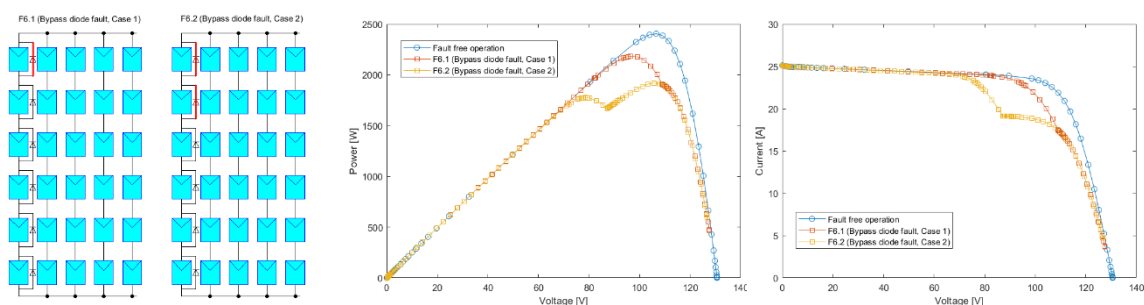
Figure 12. The PV array configuration for Bypass diode fault
