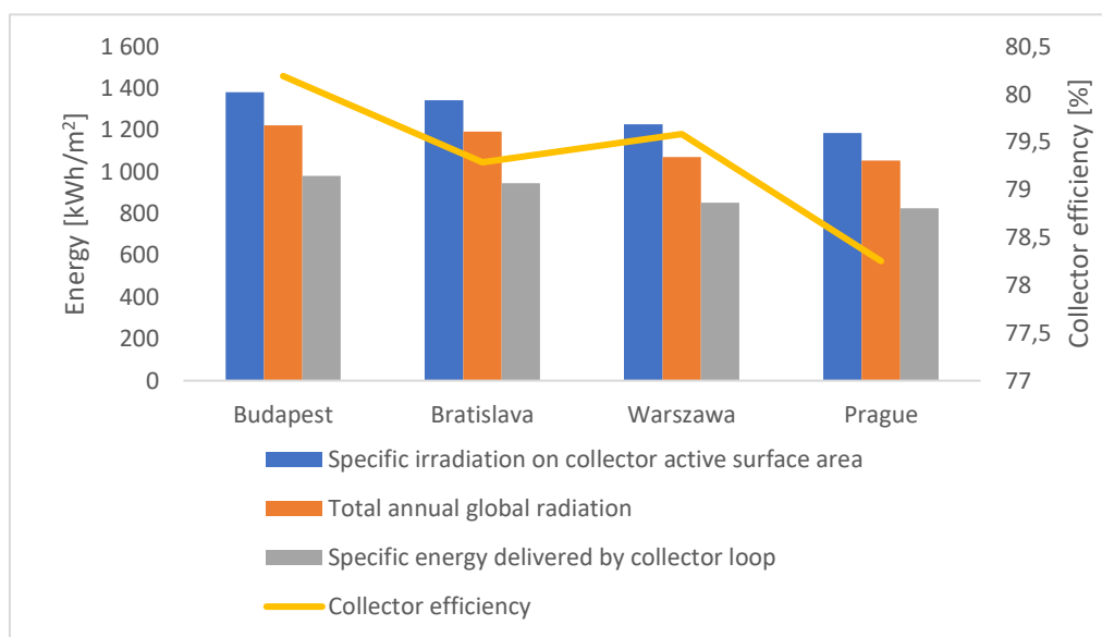
Figure 5. Analysis results in V4
