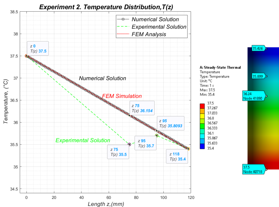
Figure 6. Temperature Distribution in steady state. B. C. 1 \rightarrow T_0 = 37.5 °C, B. C. 2 \rightarrow T_3 = 35.4 °C
