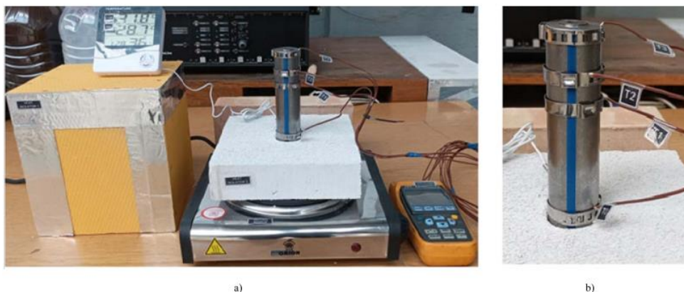
Figure 4.a) Implementation of the Experimental Rig, b) Connection of the type T-thermocouples.
