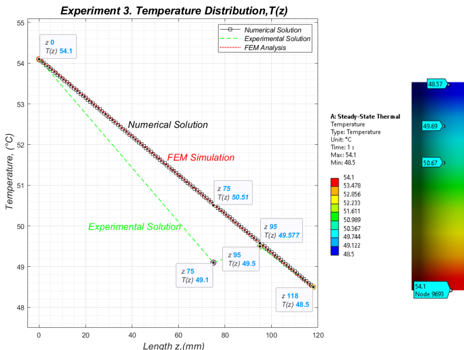
Figure 7. Temperature Distribution in steady state. B. C. 1 \rightarrow T_0 = 54.1^\circ\text{C} , B. C. 2 \rightarrow T_3 = 48.5^\circ\text{C}
