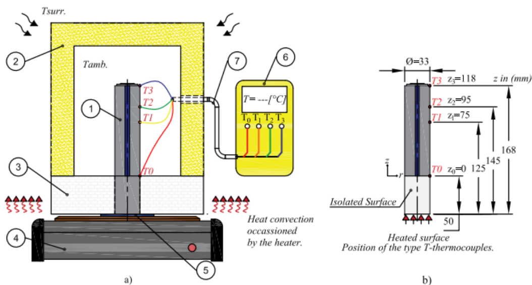
Figure 3. a) Experimental Rig, b) Position of the thermocouples Type-T
