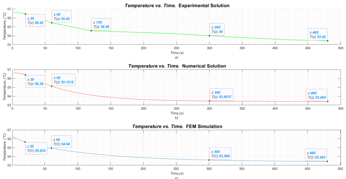
Figure 10. Temperature vs. time, a) Exp. Solution, b) F.D. Solution, c) FEM.
