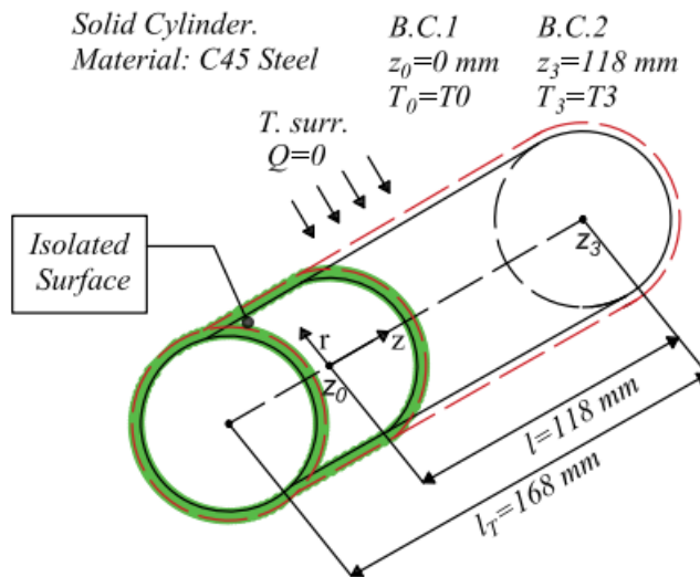
Figure 1. Heat Conduction in a solid cylinder with prescribed temperature in longitudinal direction z .
