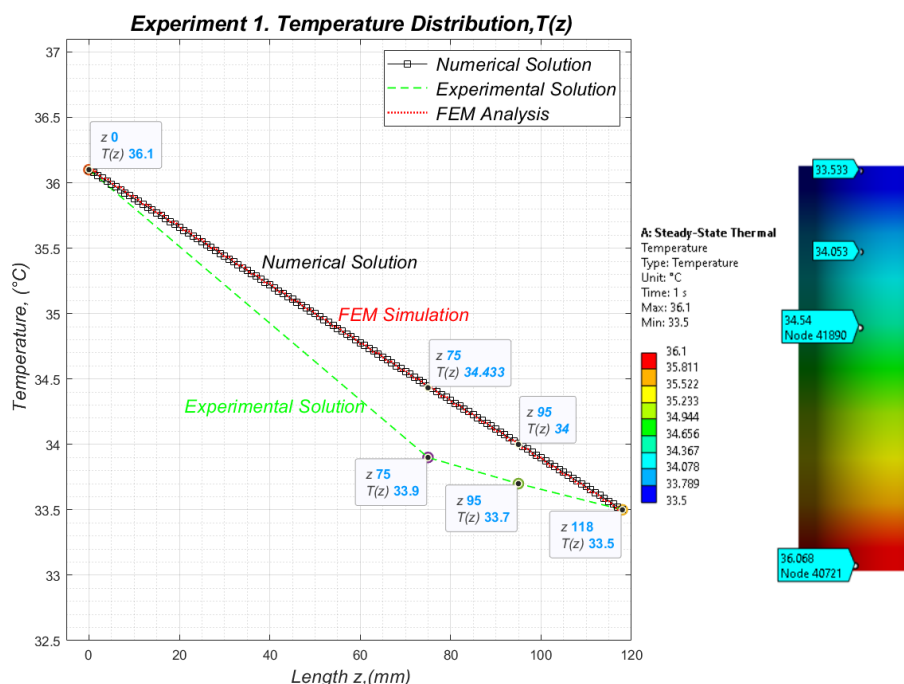
Figure 5. Temperature Distribution in steady state. B. C. 1 \rightarrow T_0 = 36.1 °C, B. C. 2 \rightarrow T_3 = 33.5 °C
