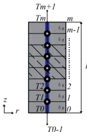
Figure 2. Finite difference approximation in the z direction of a solid cylinder.
