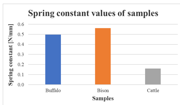
Figure 8. Values obtained for the spring constant (buffalo, bison, cattle meat)
