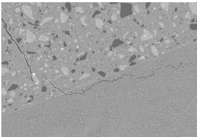
Figure 2. Picture showing the redirection of cracks when invading the SFRC core from [10]
