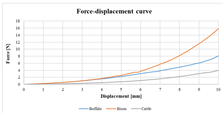
Figure 7. Force-displacement curve (buffalo, bison, cattle meat)
