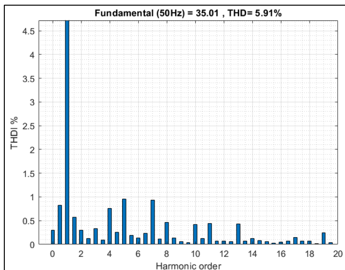
Figure 15. Total Harmonic Distortion of the current (THDI %) at irradiance 820 W / m 2
