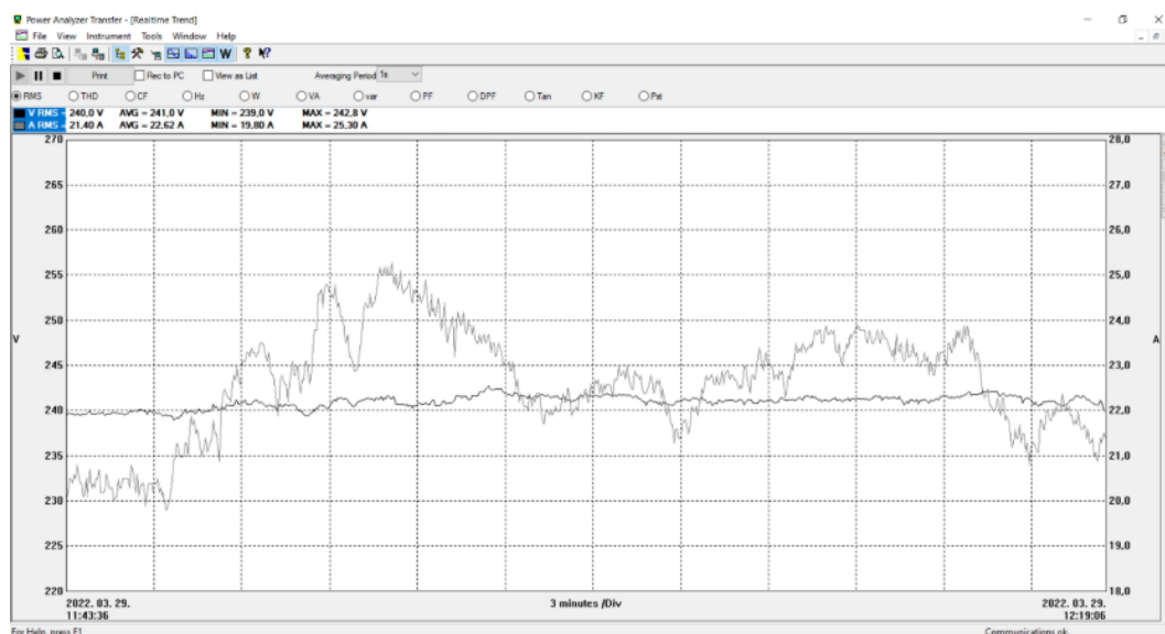
Figure 8. Trend of the RMS value of voltage and current
