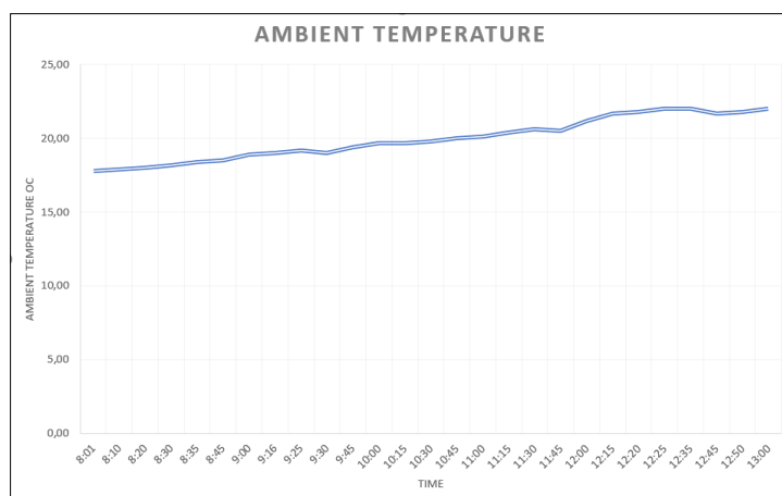
Figure 5. Ambient temperature
