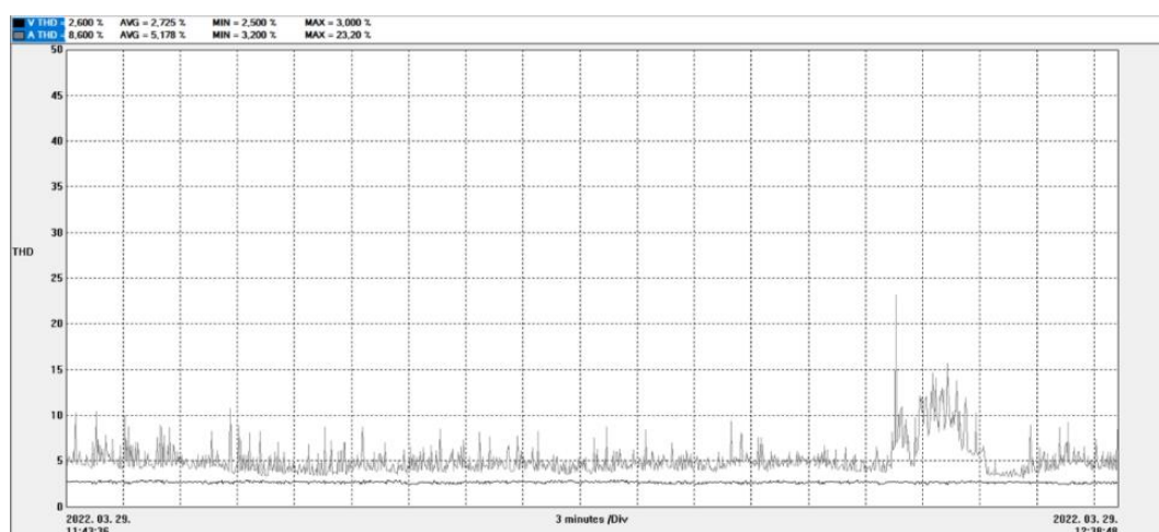
Figure 11. Shadow effect in the trend of current and voltage THD
