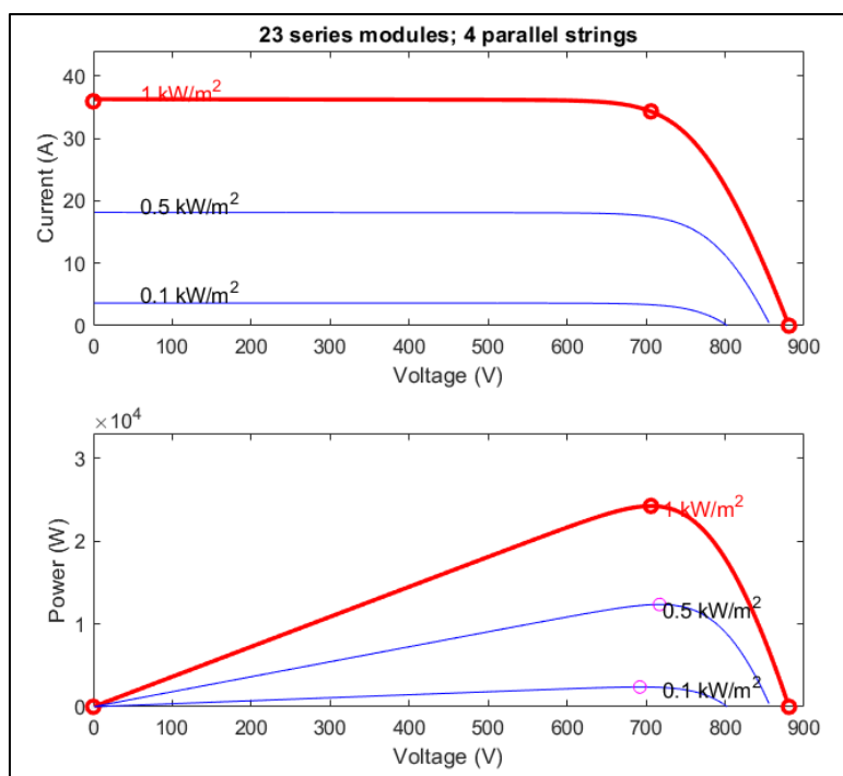
Figure 13. P–U and I–U characteristic of the PV array
