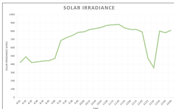
Figure 4. Solar irradiance
