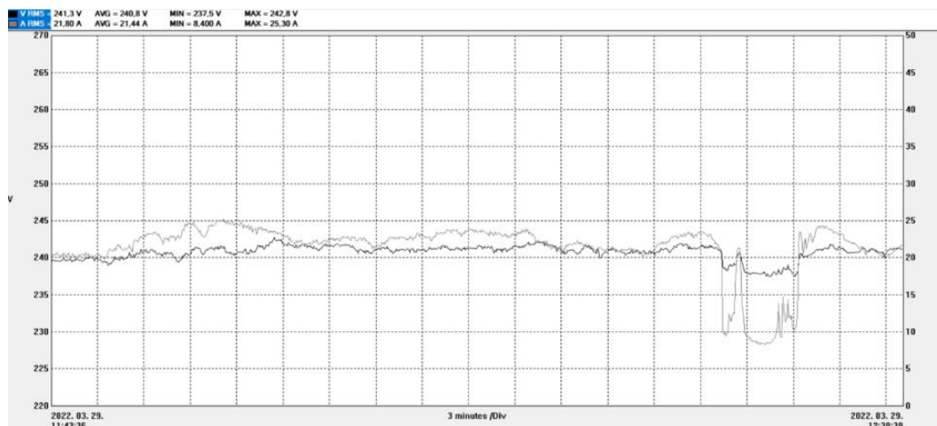
Figure 10. Shadow effect in the trend of current and voltage RMS
