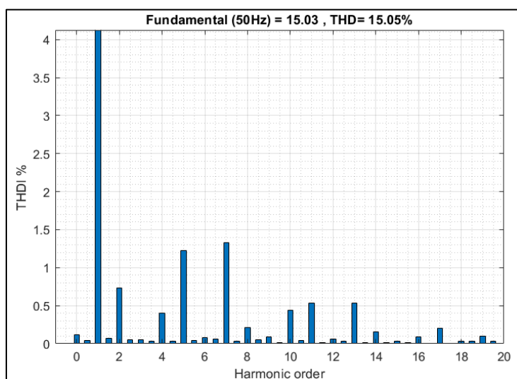
Figure 17. Total Harmonic Distortion of the current ( \text{THDI} \% ) at irradiance 350 \text{ W/m}^2
