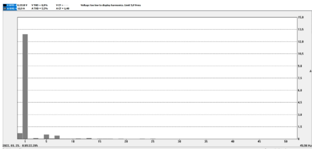
Figure 7. Harmonic components of the current in case of 260-400W/m 2 irradiance
