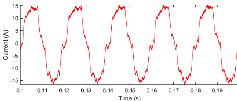
Figure 18. The sinusoidal wave of the grid current at irradiance 820 \text{ W/m}^2
