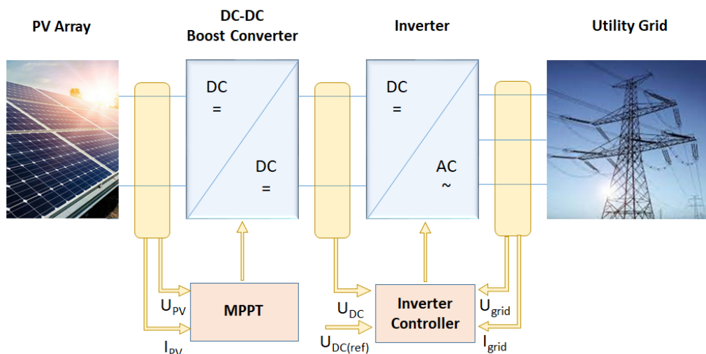
Figure 12. Structure of the simulated grid connected PV system
