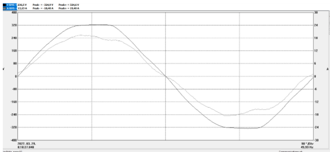
Figure 6. Waveform of voltage and current in case of 260-400W/m 2 irradiance
