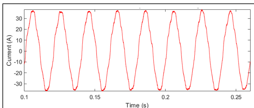
Figure 16. The sinusoidal wave of the grid current at irradiance 820 \text{ W/m}^2
