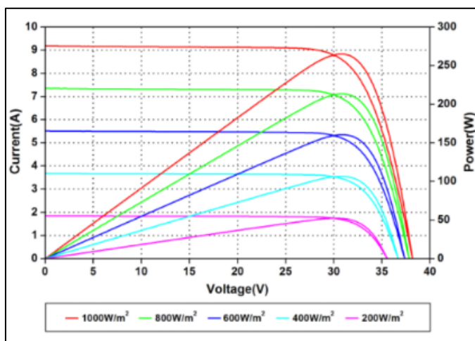
Figure 2. PV module Manufacturer curves
