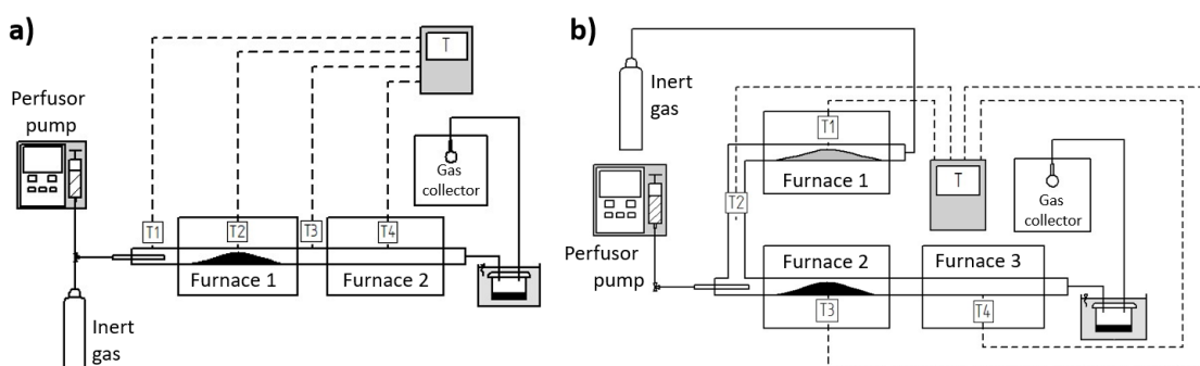
Figure 3. Sketches of a two-stage (a) and a three-stage (b) lab-scale gasification system
