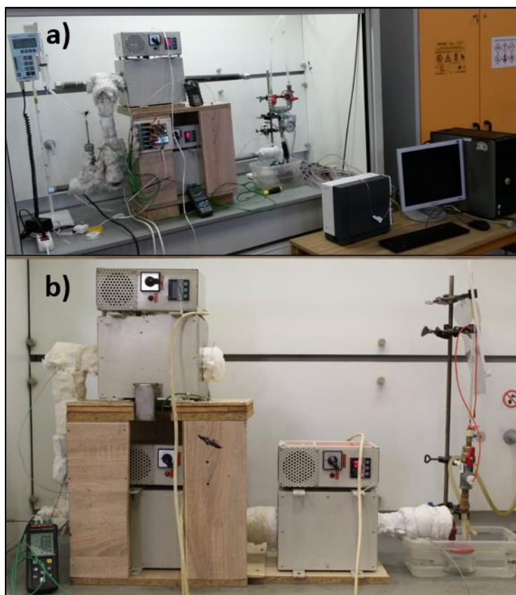
Figure 4. Photographs of a two-stage (a) and a three-stage (b) experimental gasification system
