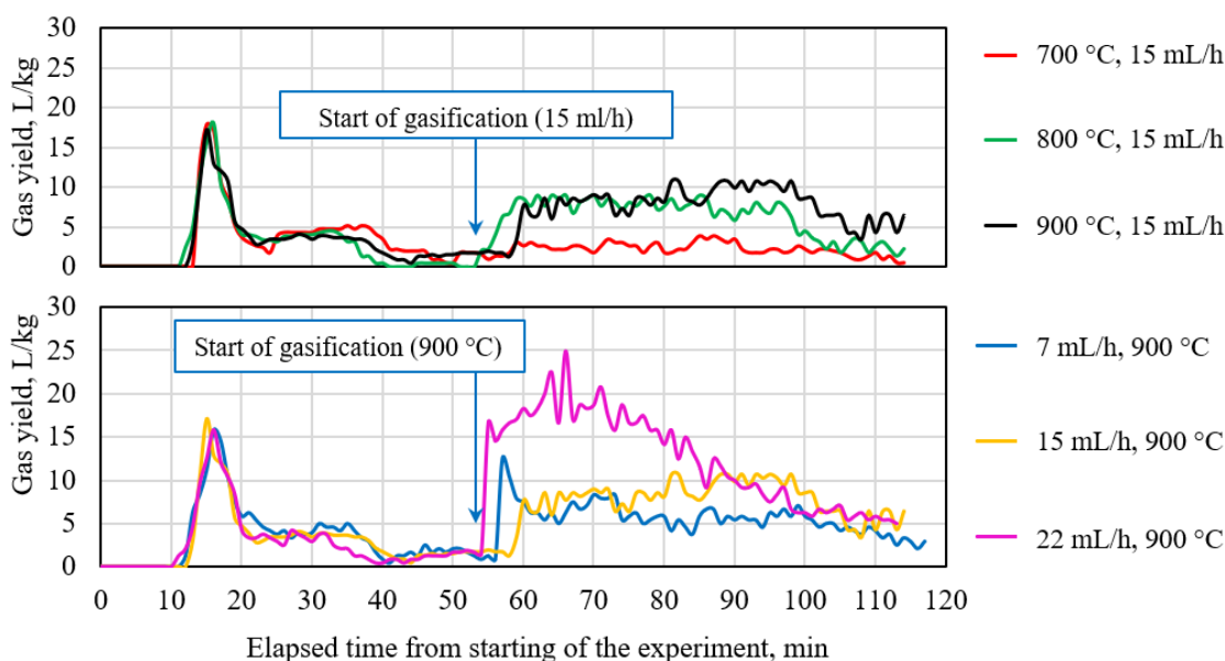
Figure 5. The changes of gas yield during the gasification of oak and canteen waste mixed in a 2:1 mass ratio
