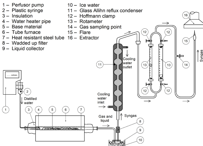
Figure 1. Schematic of the one-stage laboratory gasification system
