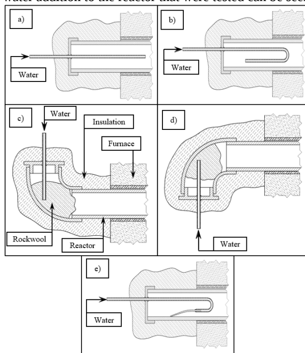
Figure 2. The tested methods for the introduction of water as a gasification medium
