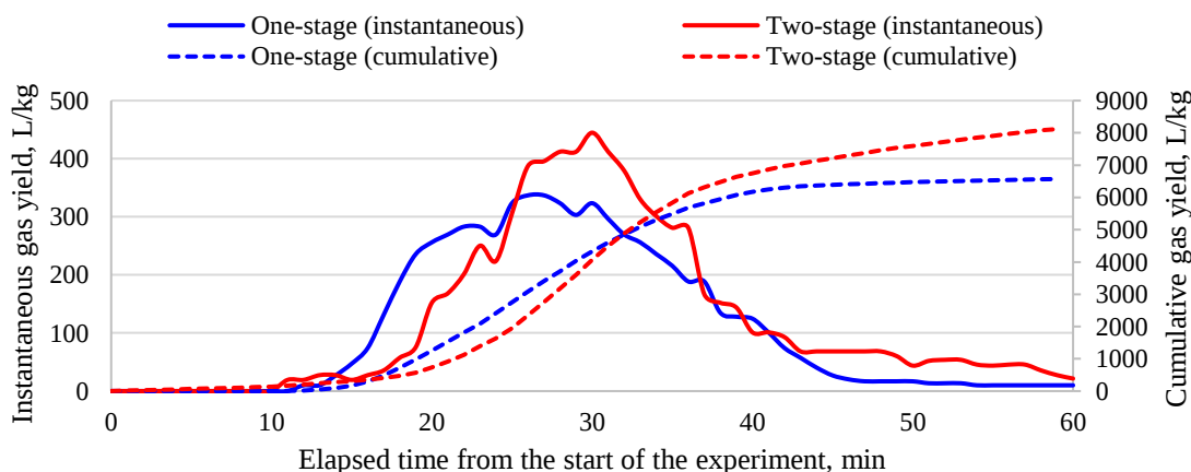
Figure 6. Instantaneous and cumulative gas yield during one- and two-stage pyrolysis of brown coal at 900 °C
