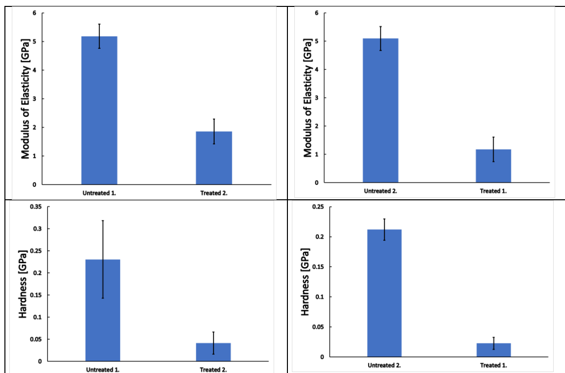
Figure 5. Mean hardness and modulus of elasticity value and standard deviation of the treated and untreated samples.
