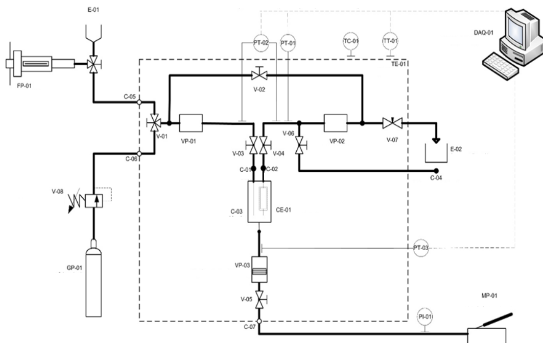
Figure 7. schematic diagram of a system operating.
