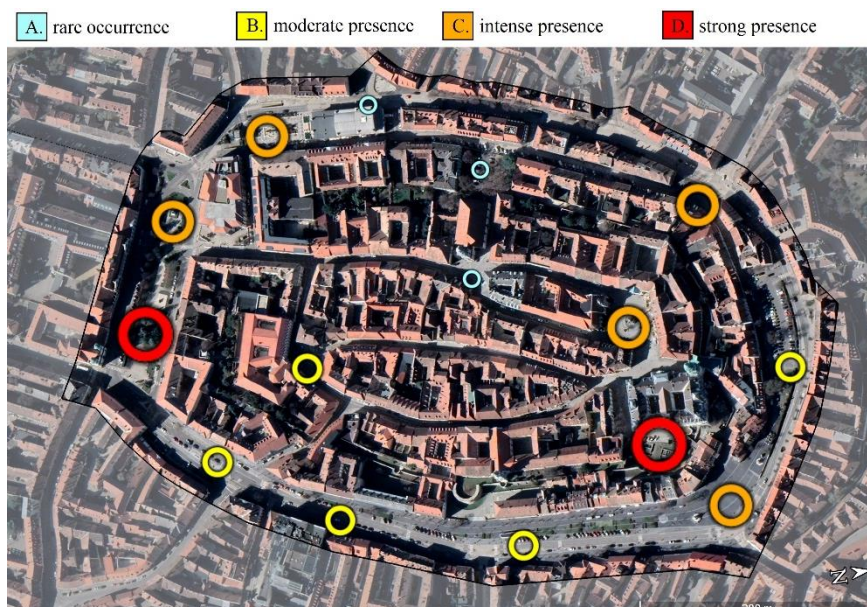
Figure 4. Pigeon abundance by groups
