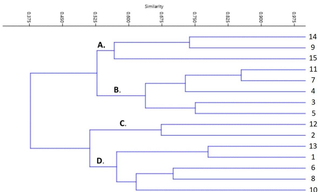
Figure 3. Classification of observation points by the number of pigeons
