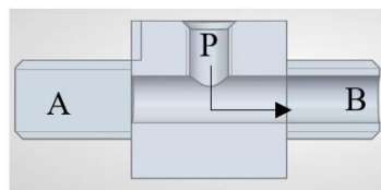
Figure 6. Muscle Connector Screw with Air Supply
