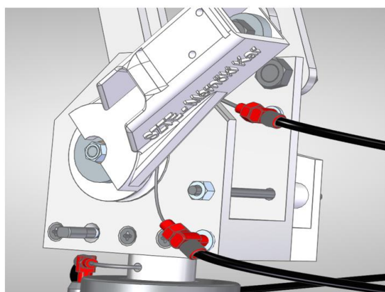
Figure 7. Bowden Housing Attachment
