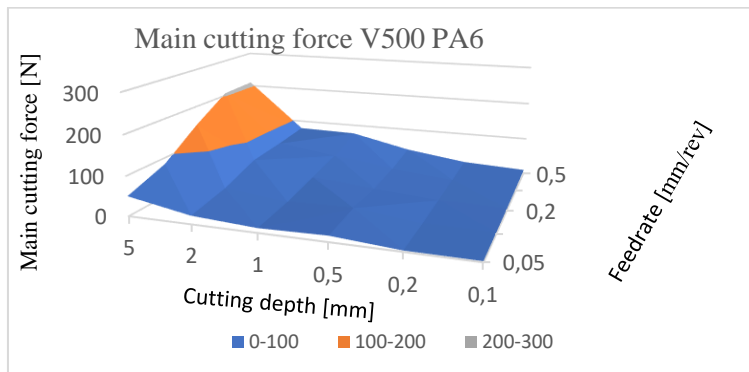
Figure 4 – The main cutting force PA6
