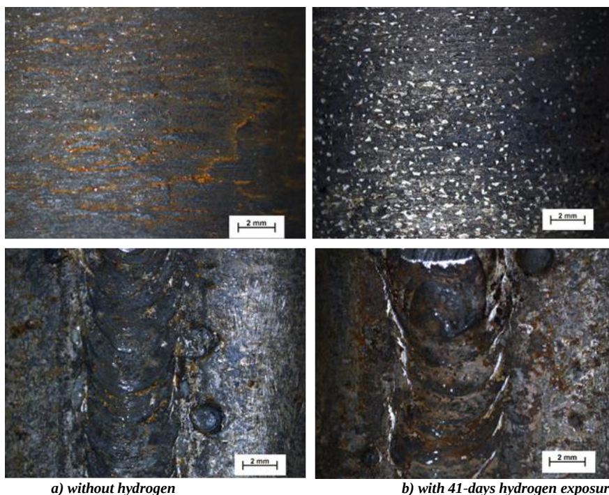
Figure 5. Macro images of the bending surfaces of the base material (on the top) and of the welded joint (bottom), N=6,5x
