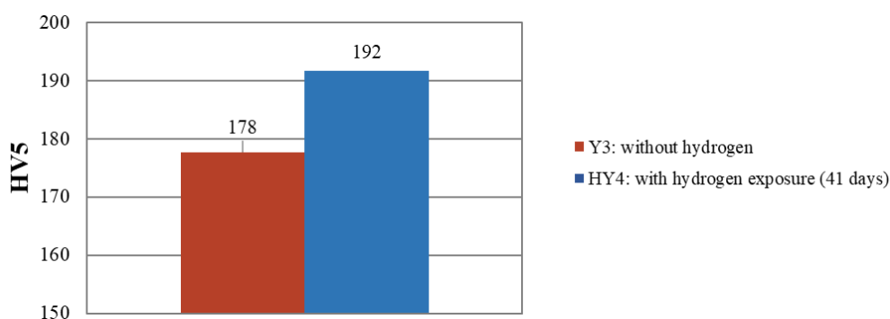
Figure 9. Average HV5 hardness values of the base materials
