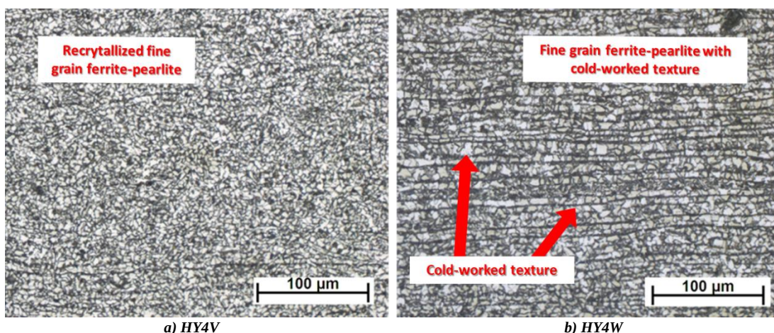
Figure 14. Recrystallized zones of the heat affected zone of welded joints, N=200\times , etched: 2% HNO_3
