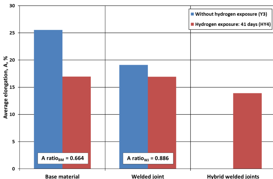
Figure 6. Influence of hydrogen exposure on the average of the elongation and the A_{ratio} values
