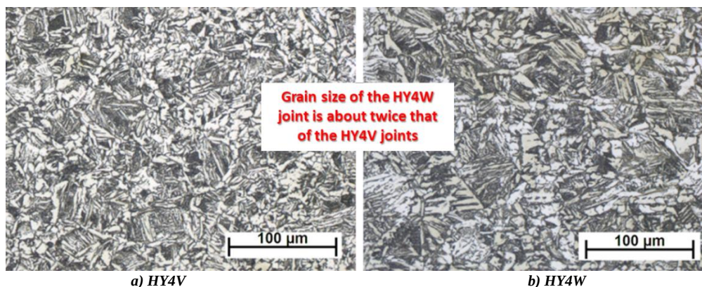
Figure 16. Coarse grained zones of the heat affected zone of welded joints, N=200\times , etched: 2% HNO_3
