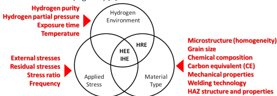
Figure 1. Classification of HEE, IHE and HRE type based on hydrogen, stress, and material factors [1]
