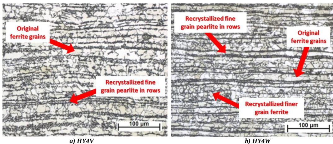
Figure 12. Intercritical zones of the heat affected zone of welded joints, N=200x, etched: 2% HNO 3
