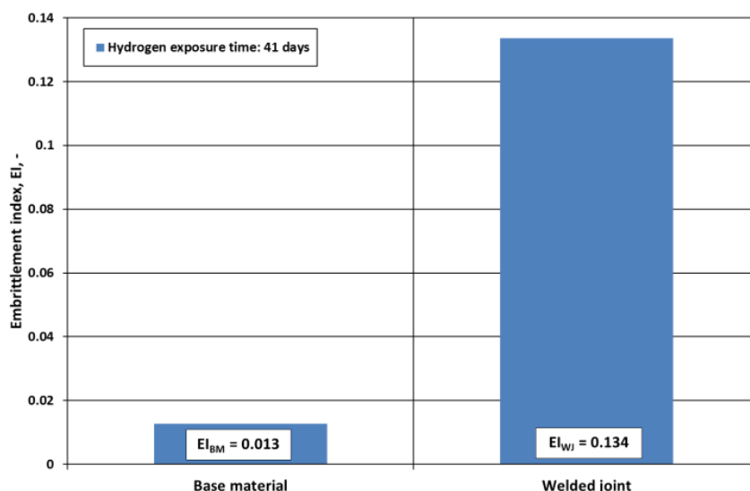
Figure 8. Embrittlement index values after 41 days of hydrogen exposure
