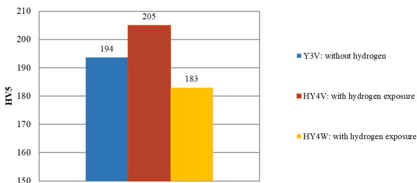
Figure 17. Results of the hardness measurement in the weld root
