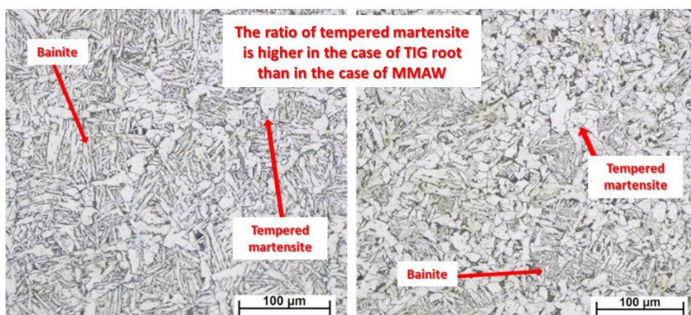
Figure 18. Roots of the welded joints, N=200\times , etched: 2% HNO_3
