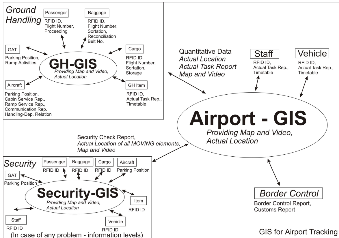
Figure 6: Airport-GIS (Source: Own Research)
