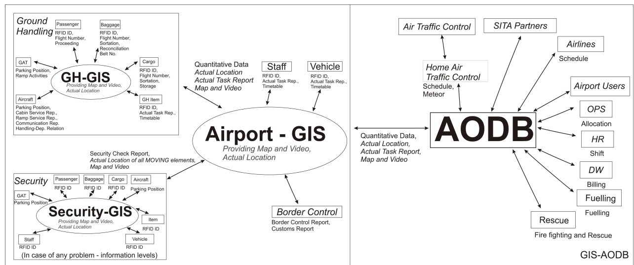
Figure 7: Airport- GIS-AODB (Source: Own Research)
