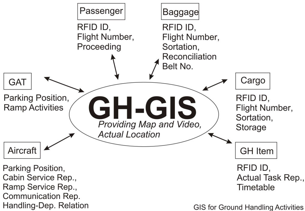
Figure 5: GIS for Ground Handling Activities (Source: Own Research)
