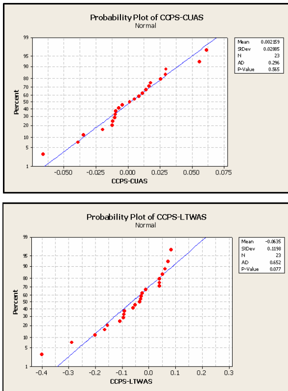
Figure 4. Probability plots of CCPS-CUAS and CCPS-LTWAS
