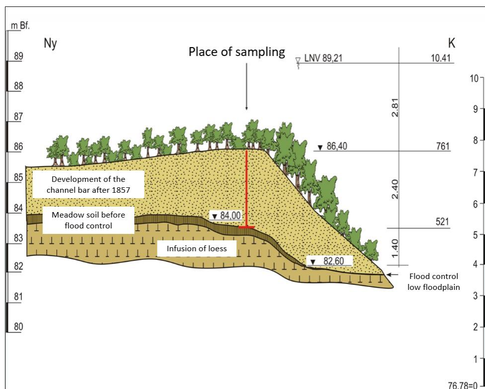
Figure 5. Development of the channel bar at Szolnok 7
