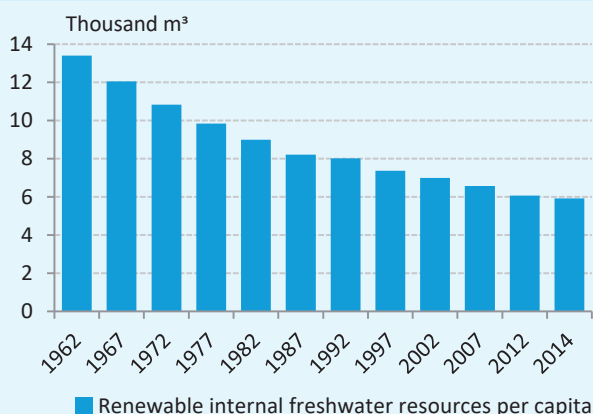
Chart 1-17: Renewable internal fresh water resources per person
