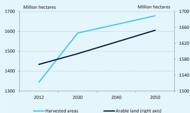
Chart 4-13: Forecast for harvested and arable land based on the green growth scenario
