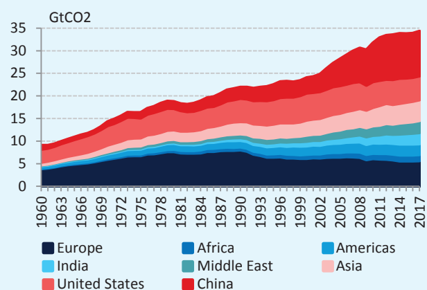
Chart 1-13: Carbon dioxide emissions by country/region
