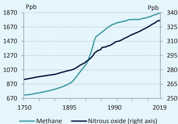
Chart 1-7: Atmospheric concentration of methane and nitrous oxide
