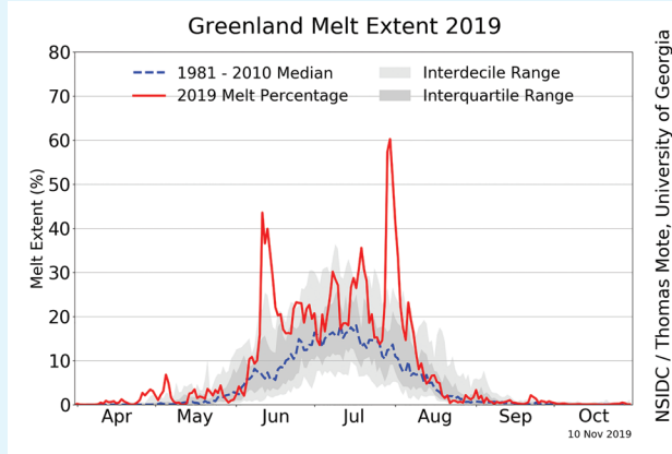
Chart 1-14: Extent of ice sheet melting in Greenland
