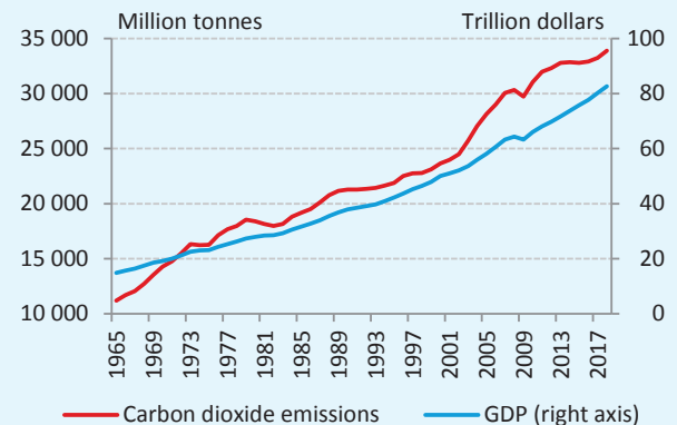
Chart 1-5: Global GDP and global carbon dioxide emissions
