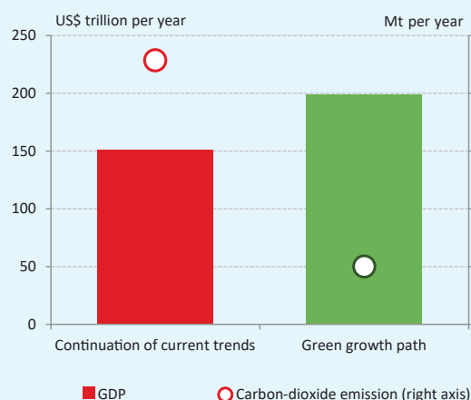
Chart 2-9: Real GDP and CO 2 emissions in the case of continuation of the present trends and in the green growth scenario in 2050
