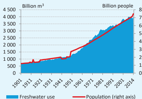
Chart 1-16: Fresh water consumption and population
