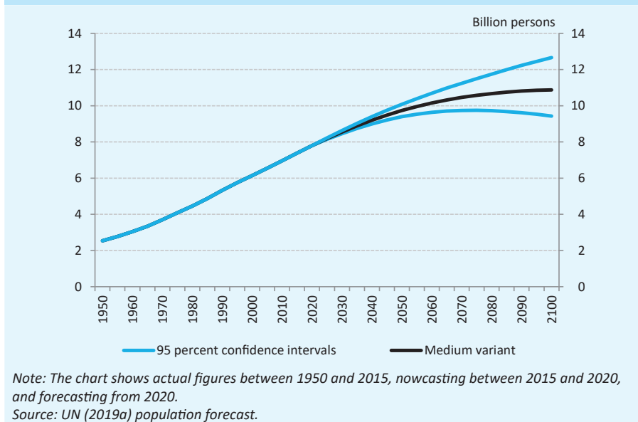
Chart 6-11: Global population based on the medium variant and the 95 percent confidence interval thereof
