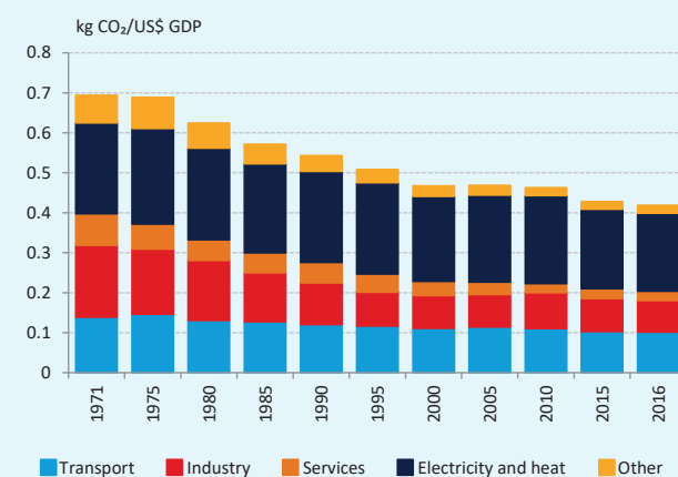
Chart 2-6: CO 2 emission by sector as a percentage of GDP, 1971–2016
