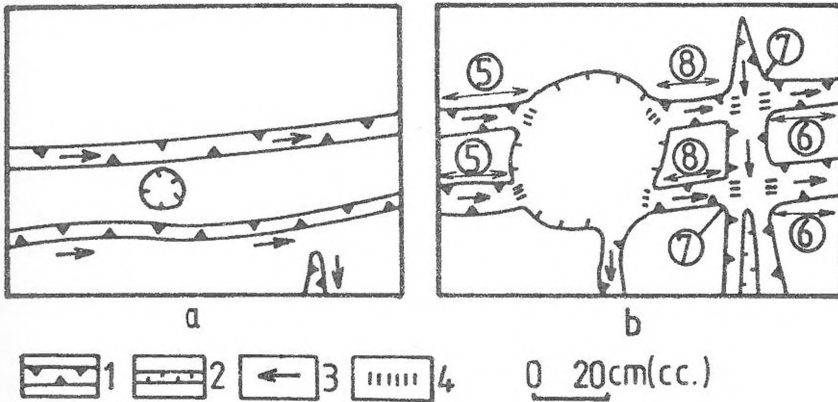
Fig. 8: Beheading by solution pan and trough-crossing (after sketch and photo)
