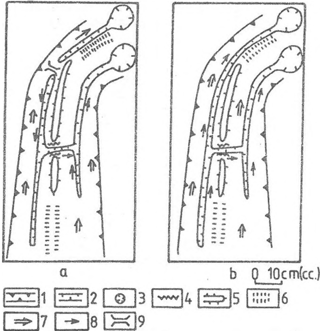
Fig. 10: Simple(a) and composite beheading (after sketch and photo) Legend: 1: edge of type I trough, 2: edge of type III trough, 3: pit, 4: diagonal canyon, 5: inter-trough crest, 6: rise between the troughs, 7: slope of the type I trough, 8: slope of the type III trough, 9: trough-bottom watershed
