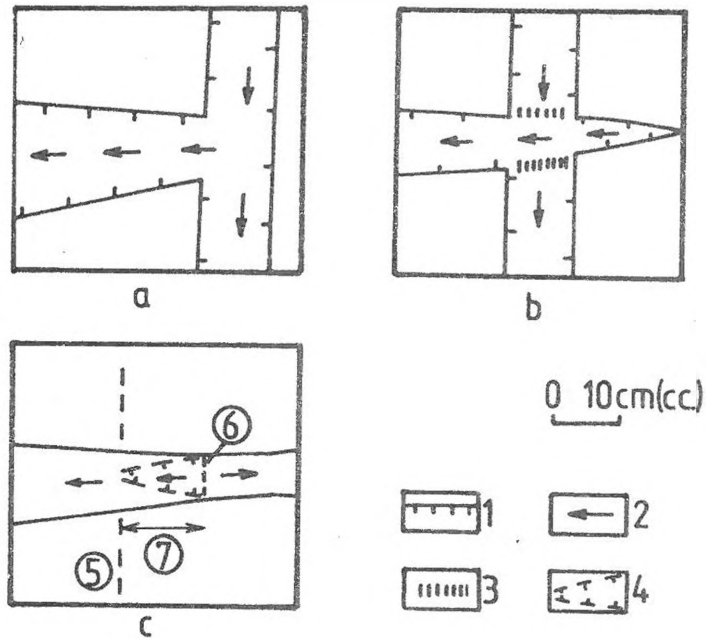
Fig 7: Trough beheadings by regression (after photos)
