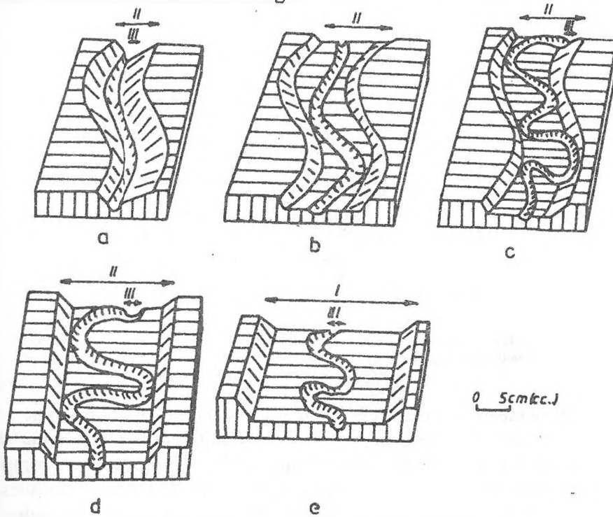
Fig. 4: Inherited meanders of composite karren troughs
