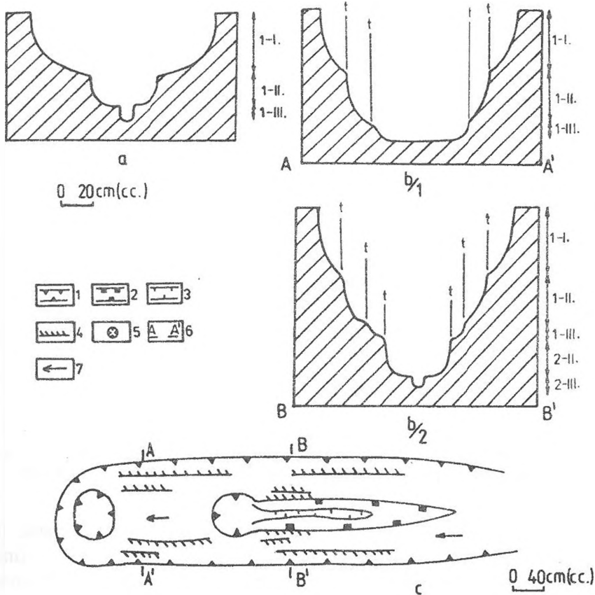
Fig 12: Terrace development in the case of piracy (after survey, sketch and photo) Legend: a: stage of development before piracy, b: stage of development after piracy, b/1: inactive trough section after the second location of beheading, b/2: active trough section after the second location of beheading, c: plan, I, II, III trough types on the cross sections. 1: edge of the 1-I trough, 2: edge of the 2-II trough, 3: edge of the 2-III trough, 4: terrace, terrace remnant, 5: pit, 6: location of section on the plan, 7: slope of the trough-bottom.
