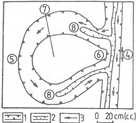
Fig 5: The beheading of a bend (after a photograph) Legend: 1: type I trough, 2: type III trough, 3: direction of the fall of the trough-bottom, 4: location of beheading, 5: karren trough oxbow, 6: karren trough neck 7: karren trough inselberg, 8: retreating troughs
