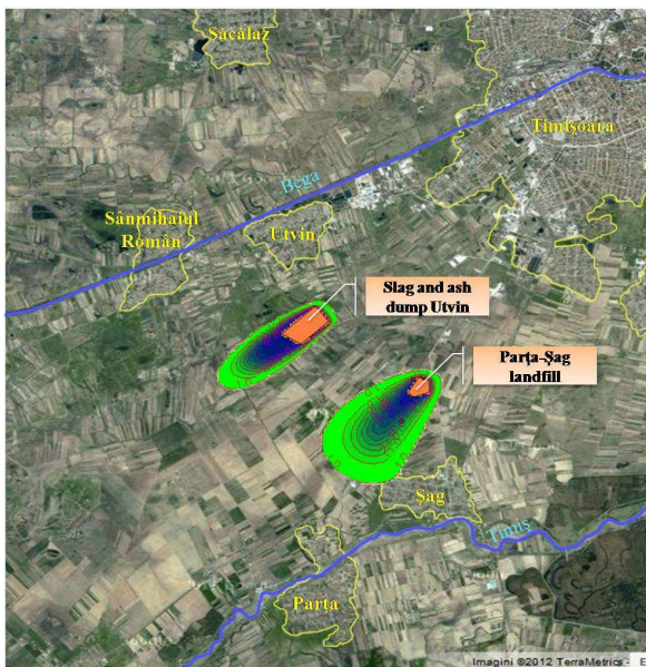
Figure 4. Pollution plum 2023 (35 years slag and ash dump Uvin; 50 years Parța-Șag landfill)
