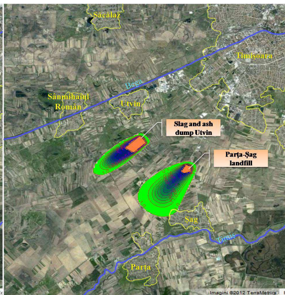
Figure 5. Pollution plum 2033 (45 years slag and ash dump Uvin; 60 years Parța-Șag landfill)
