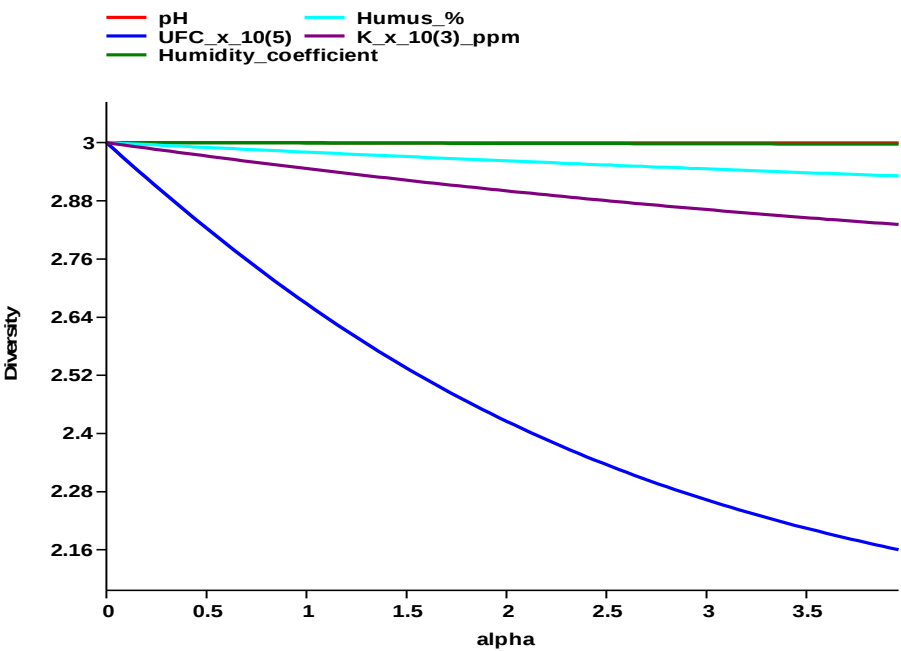
Figure 2. Diversity profiles
