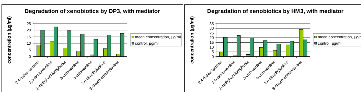
Figure 2. Degradation of xenobiotics by DP3 and HM3 strains after guaiacol addition
