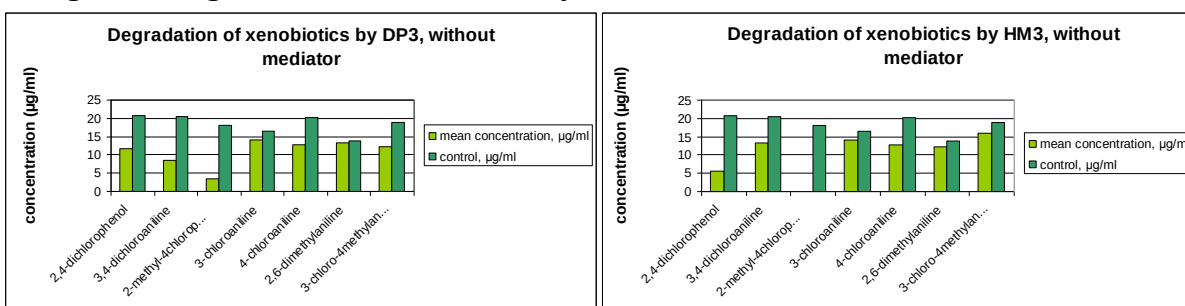
Figure 1. Degradation of xenobiotics by DP3 and HM3 strains without a mediator
