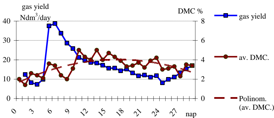
Figure 2. Gas production and dry matter content in the fermentor with average 3,4% DMC
