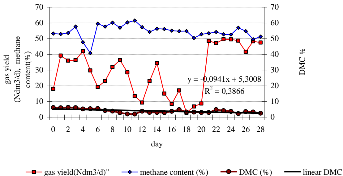
Figure 3. Gas production and dry matter content in the fermentor with average 4,6% DMC
