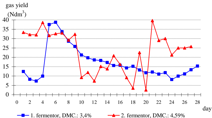
Figure 1. Gas production in the control fermentors
