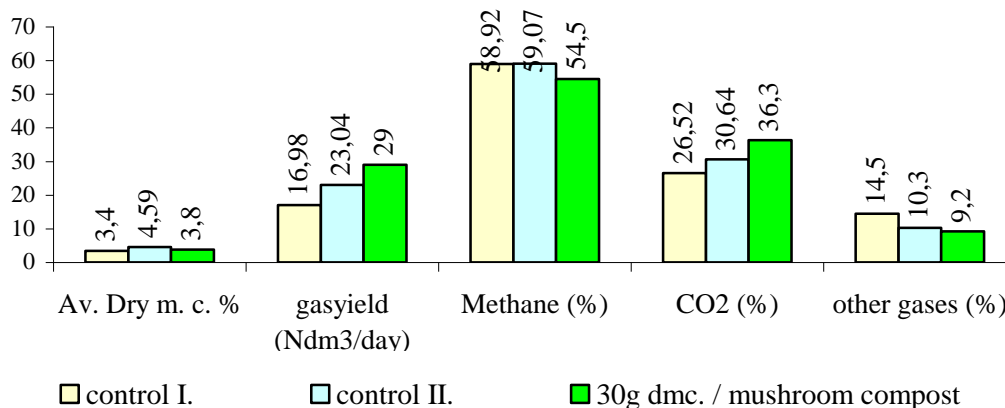
Figure 5. Average gas development parameters on liquid pig manure basis, yielded mushroom compost dosed
