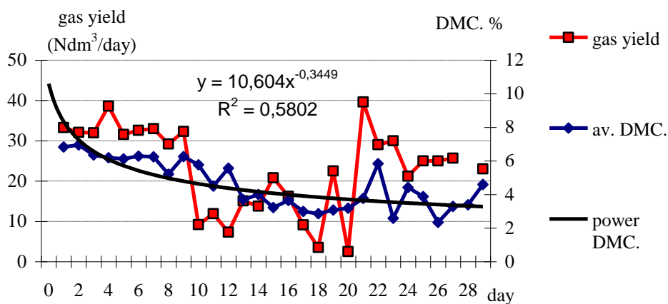
Figure 2. Gas production and dry matter content in the fermentor with average 3,4% DMC
