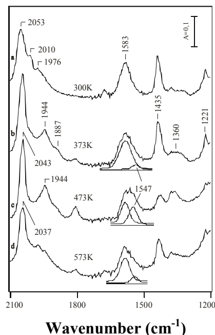
Figure 4. FTIR spectra of Re/TiO 2 following the adsorption of \text{H}_2 + \text{CO}_2 (1:1) at different temperatures for 15 min ( T_R=673\text{ K} )
