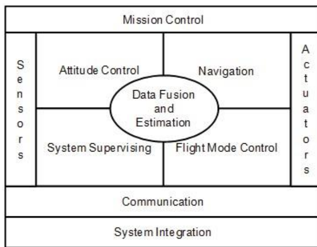
Figure 5. Software structure
