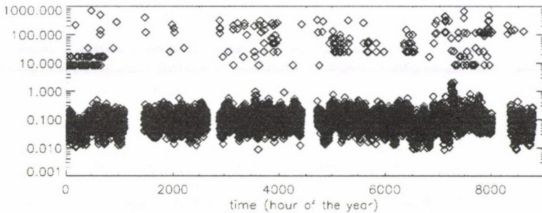
Fig. 2. Maximum amplitude in Pc3 activity versus time in lin-log scale
