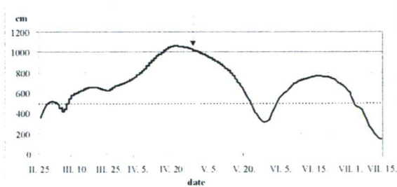
Fig. 2 Recorded water level at the Mindszent fluvio-meter in 2006 (data: www.vizadat.hu ). The arrow indicates flow velocity measure date
