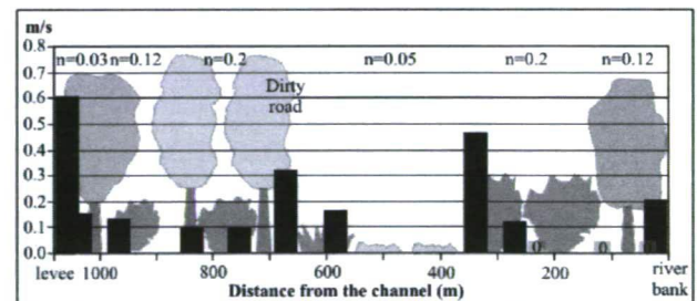
Fig. 4 Flow velocity distribution of the cross-section M 1-13 (the vegetation type and the roughness are also indicated)
