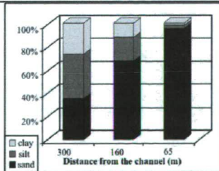
Fig. 10 Aggradation along the cross-section MI-11 and the grain size distribution of sediment
