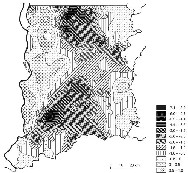
Fig. 4 The level of groundwater in March 2003 (in relation to the average of 1971-1975)
