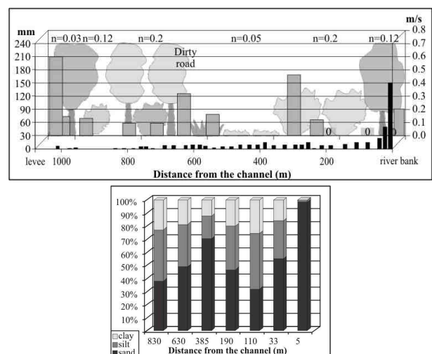
Fig. 13 Aggradation along the cross-section Ml-13 and the grain size distribution of sediment
