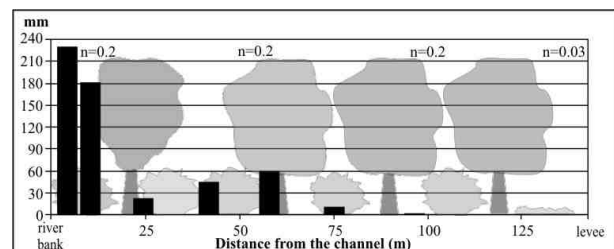
Fig. 12 Aggradation along the cross-section Mr-7
