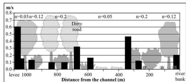
Fig. 4 Flow velocity distribution of the cross-section M l-13 (the vegetation type and the roughness are also indicated)
