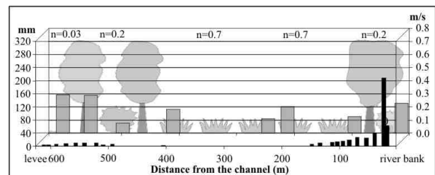
Fig. 11 Aggradation along the cross-section Ml-3
