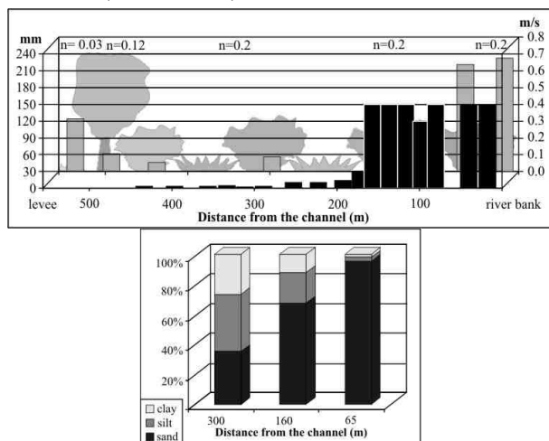
Fig. 10 Aggradation along the cross-section Ml-11 and the grain size distribution of sediment
