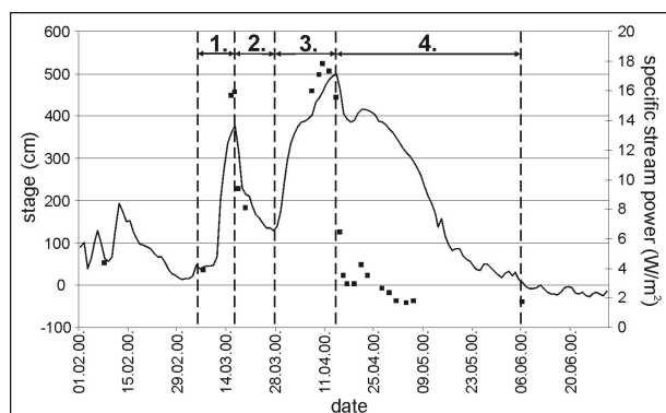
Fig. 4 Hydrograph (solid line) and calculated data of specific stream power (squares) at the Makó cross-section (Maros). Black squares also indicate dates of channel cross-sectional measurements. Phases of floods are indicated as 1-4
