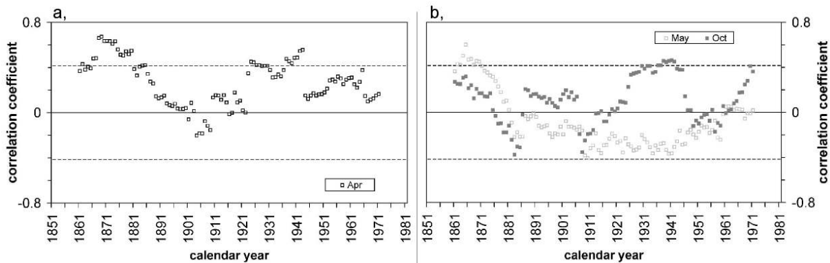
Fig. 5 Fluctuation of coefficients of 21yrs moving window correlation computed between radiodensitometric indices of Novaci spruce samples, and a few arbitrary chosen monthly mean temperature targets from the Sibiu record. a: maximum density vs. April, b: minimum density vs. May (open squares) and October (filled squares). Dashed horizontal lines denote the 95% significance levels
