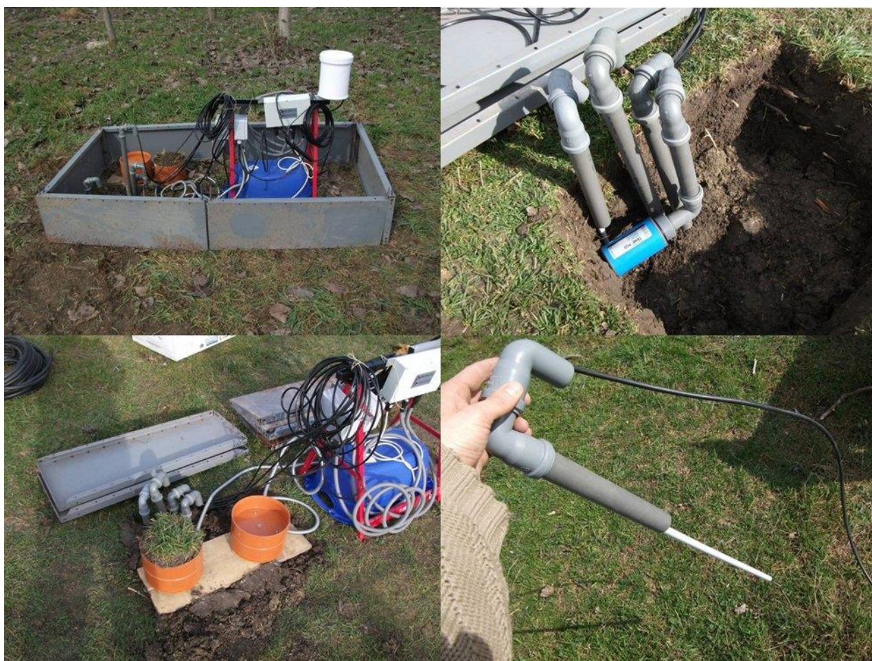
Fig. 2 Installation of the measurement stations
